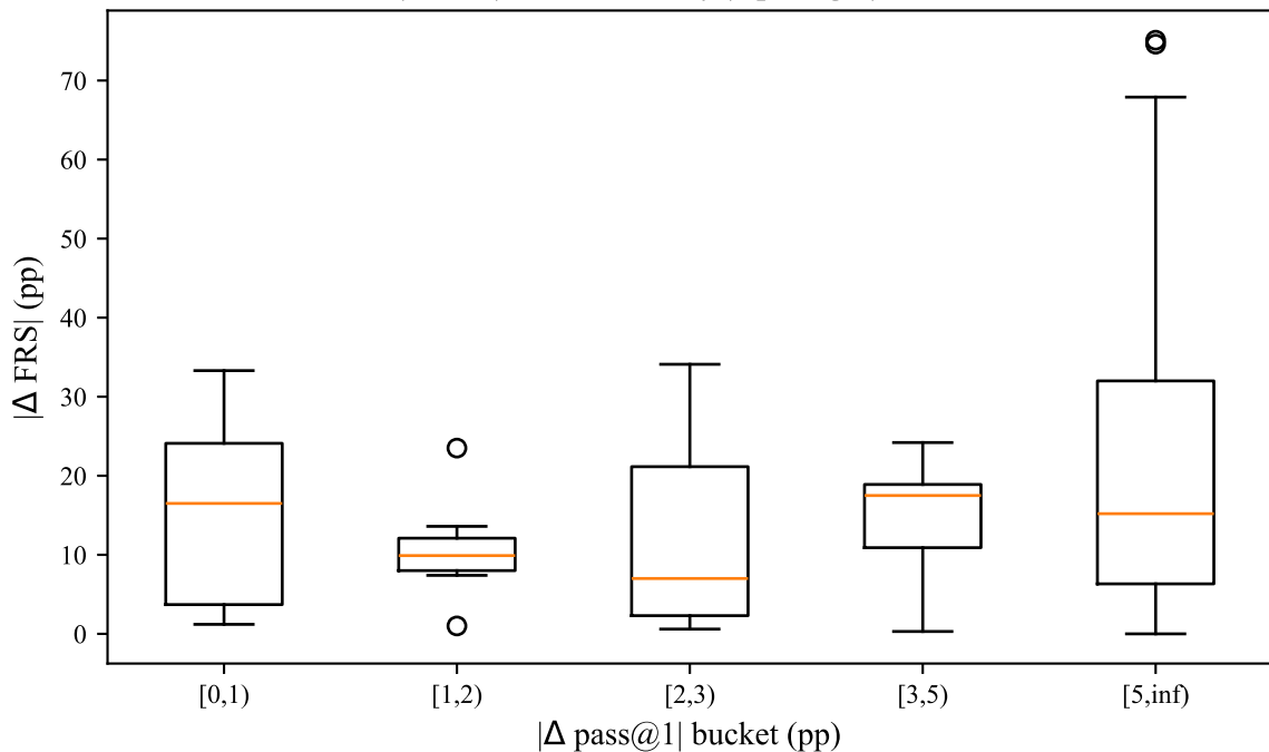
|\Delta \text{FRS}| distribution by |\Delta \text{pass}@1| bucket
