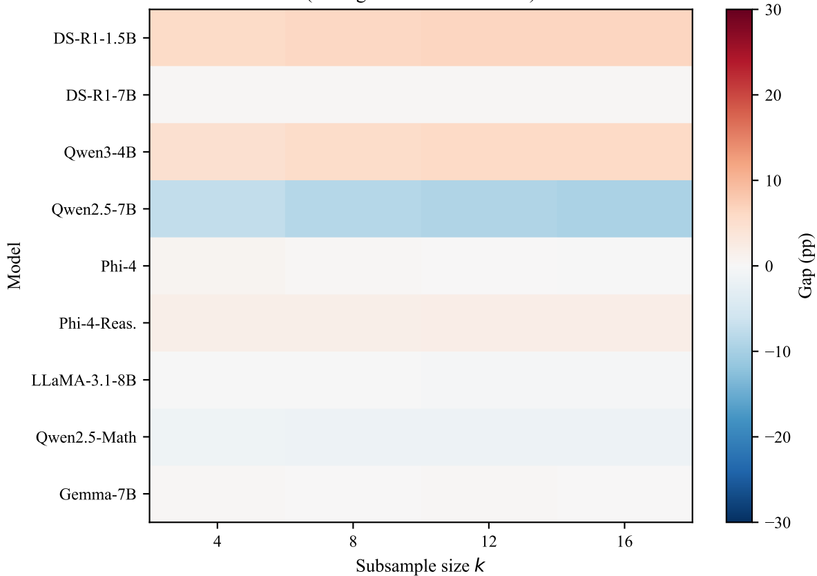
Mean accuracy gap (confident — unconfident half), pp (averaged over benchmarks)
