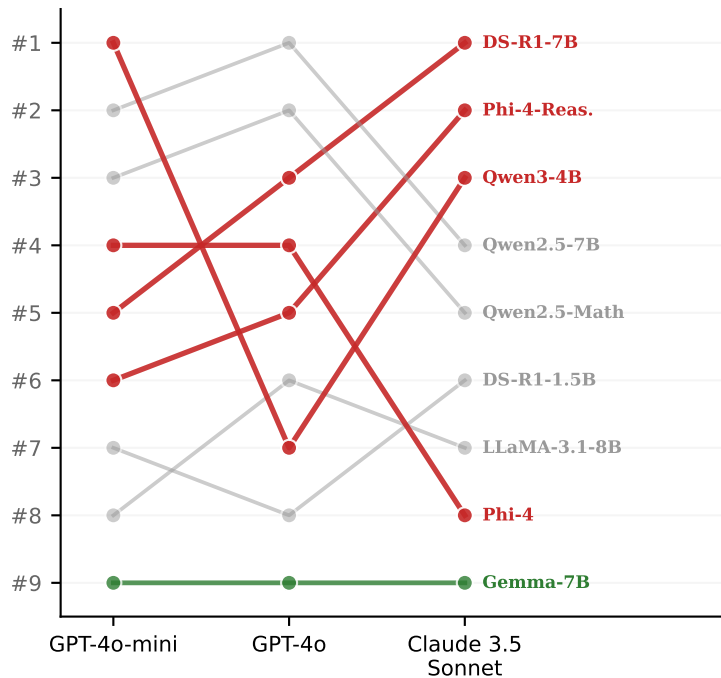
(b) Model rank by judge (green=stable, red=unstable)
