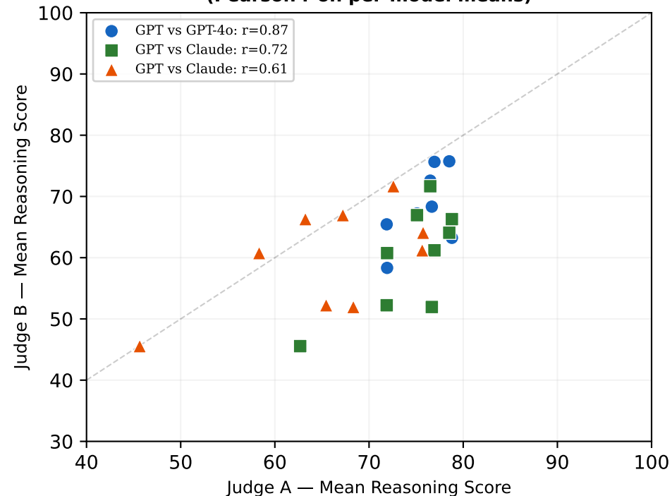
(a) Score correlation across judges (Pearson r on per-model means)
