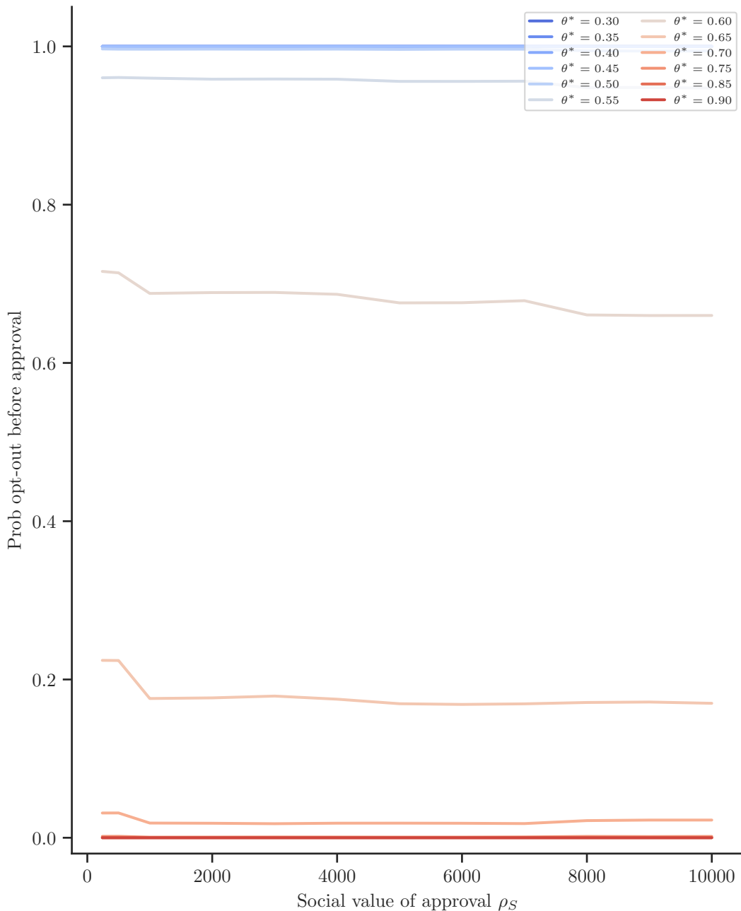
True opt-out probability vs \rho_S for each theta star
