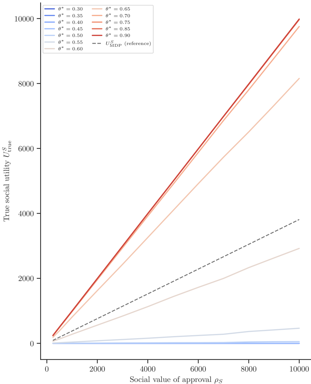
True social utility vs \rho_S for each \theta^*
