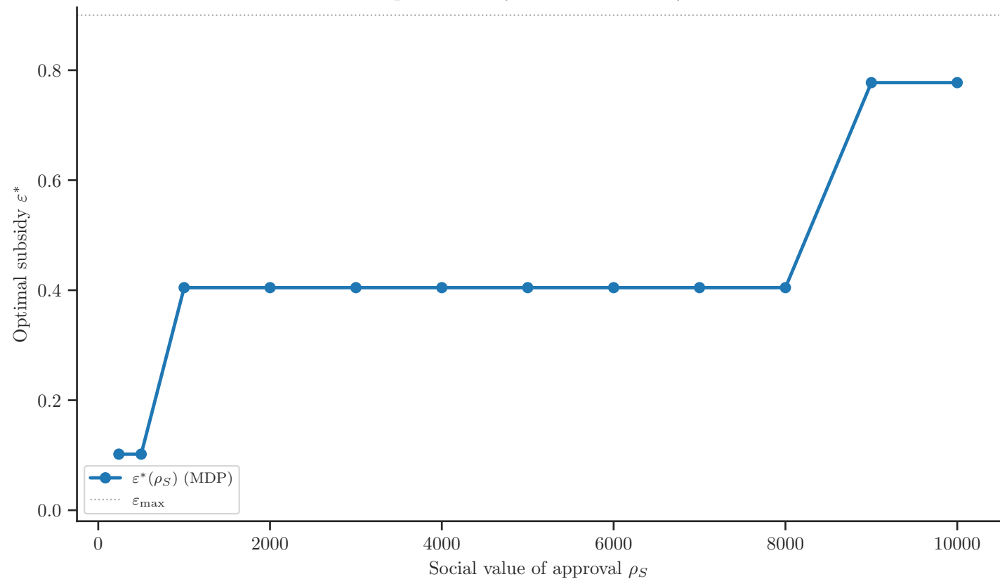
Optimal subsidy \varepsilon^* as a function of \rho_S
