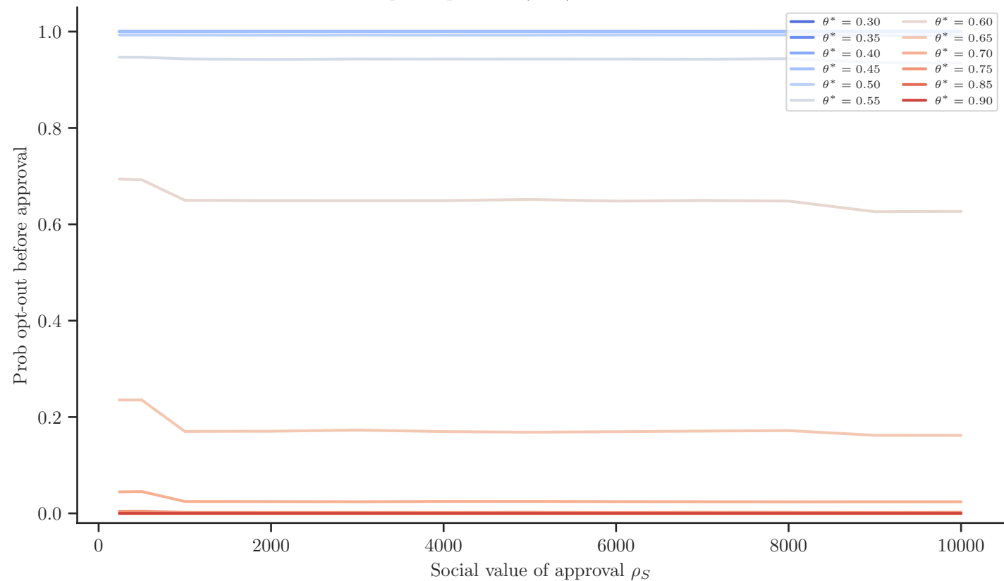
True opt-out probability vs \rho_S for each theta star
