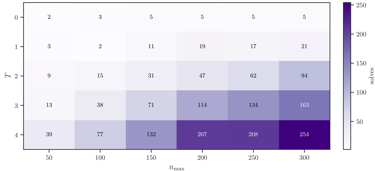
Total MDP solves — fiducial \rho_S, \theta^*
