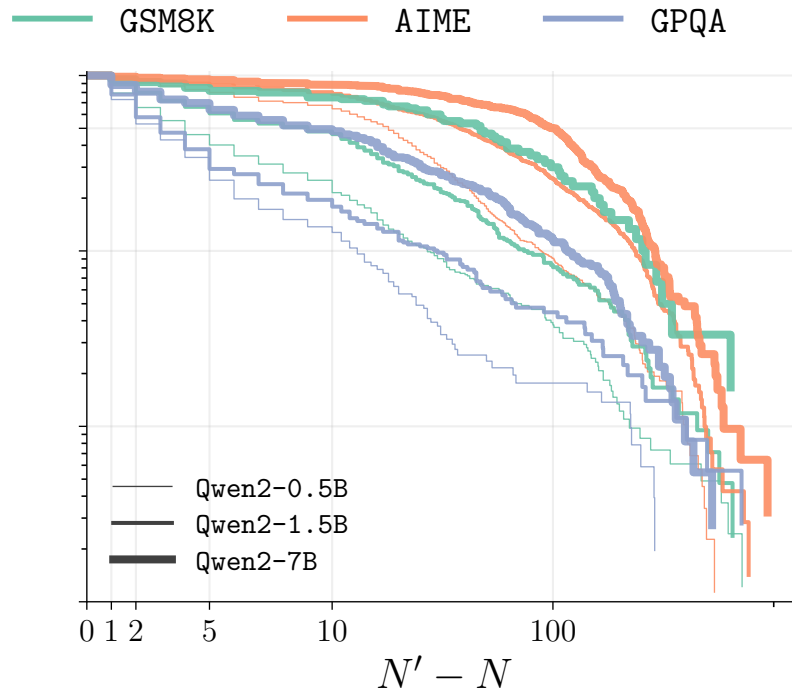
(b) Qwen models
