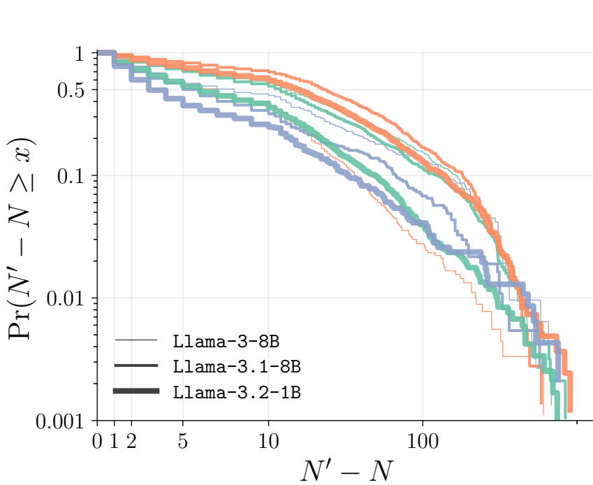
(a) Llama models
