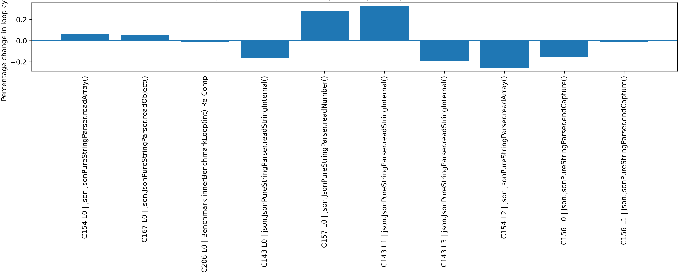
Json: NoNested vs Nested (percentage change, baseline = Nested)
