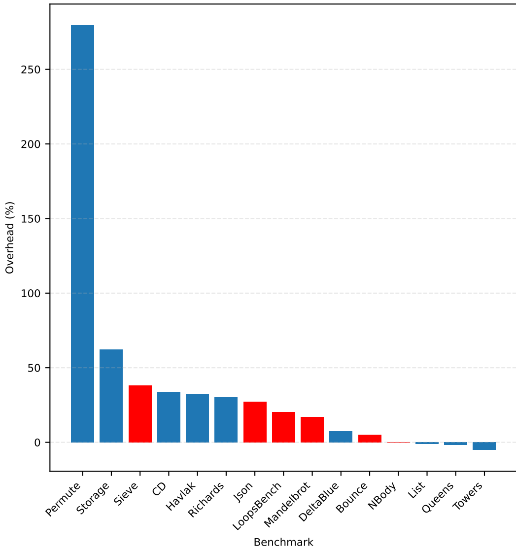
BuBoL's Overhead per Benchmark
