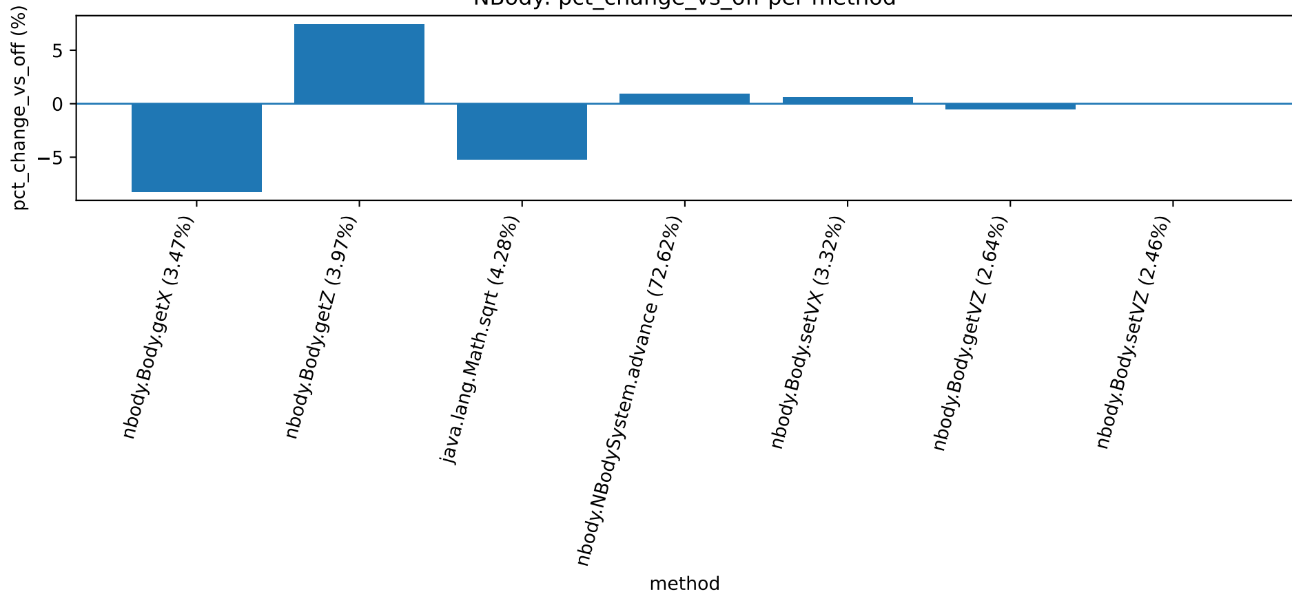
NBody: pct_change_vs_off per method
