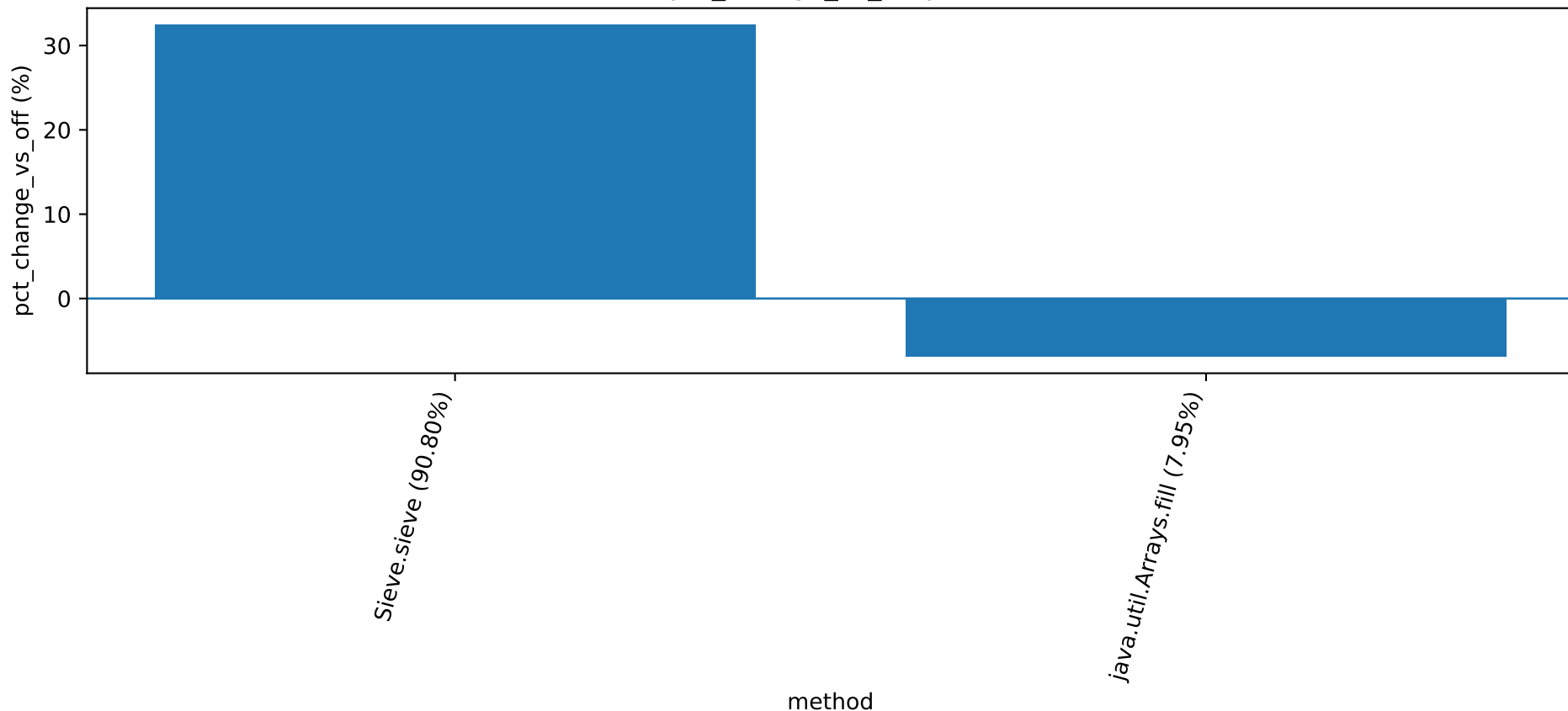
Sieve: pct_change_vs_off per method
