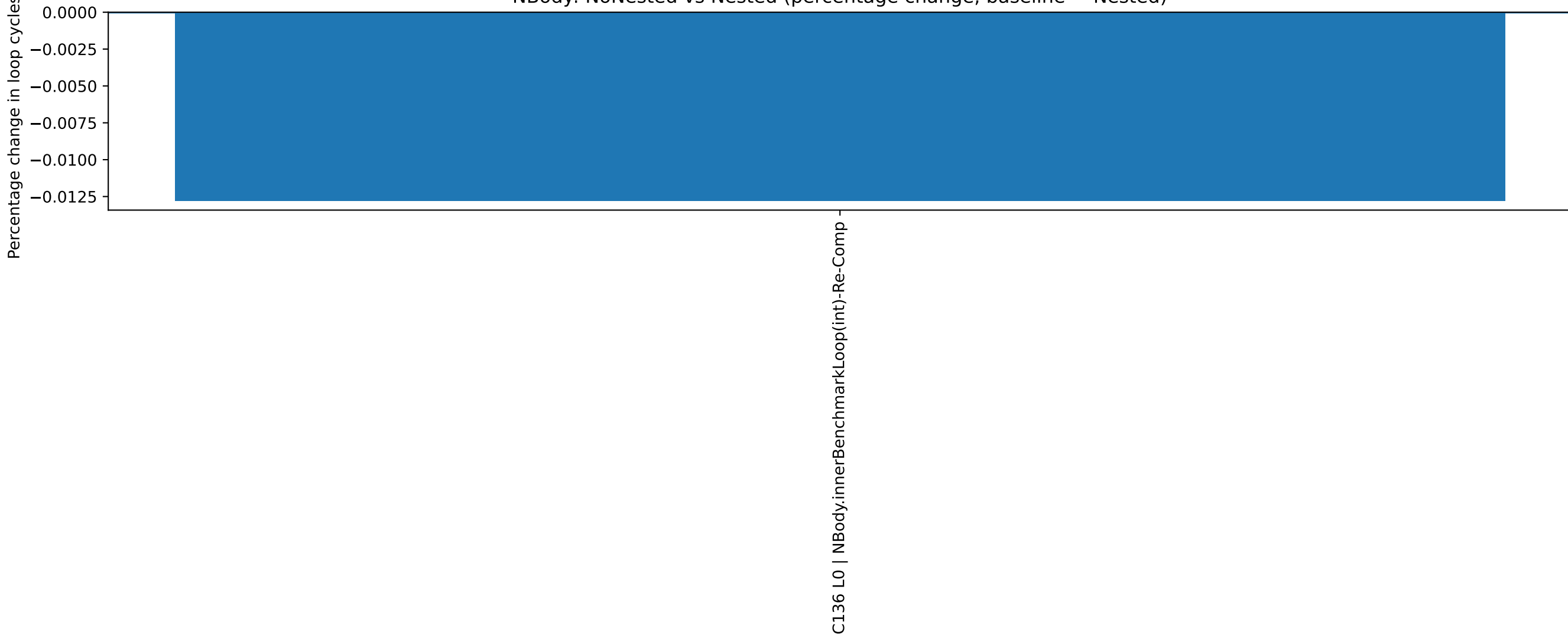
NBody: NoNested vs Nested (percentage change, baseline = Nested)
