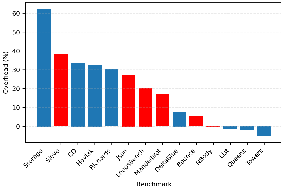
BuboL's Overhead per Benchmark
