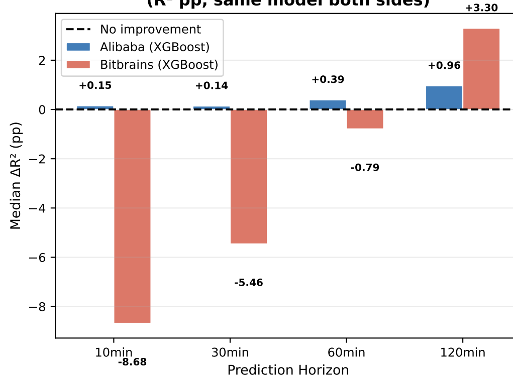
XGBoost ML Improvement over Naive ( R^2 pp, same model both sides)
