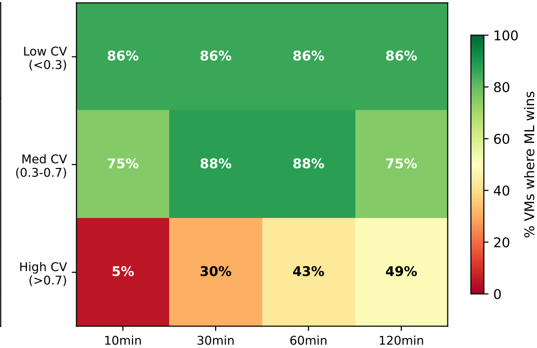
ML Win Rate by CV Bin × Horizon (Bitbrains active VMs)
