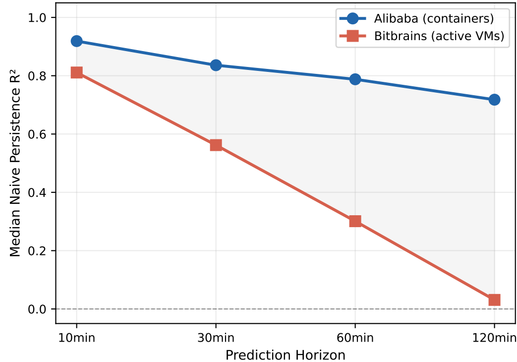
Naive Baseline Degradation with Prediction Horizon
