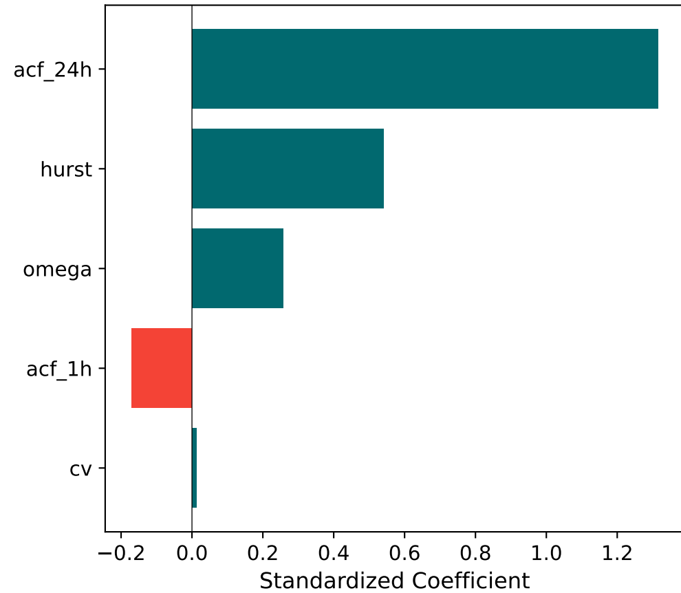
Feature Importance
