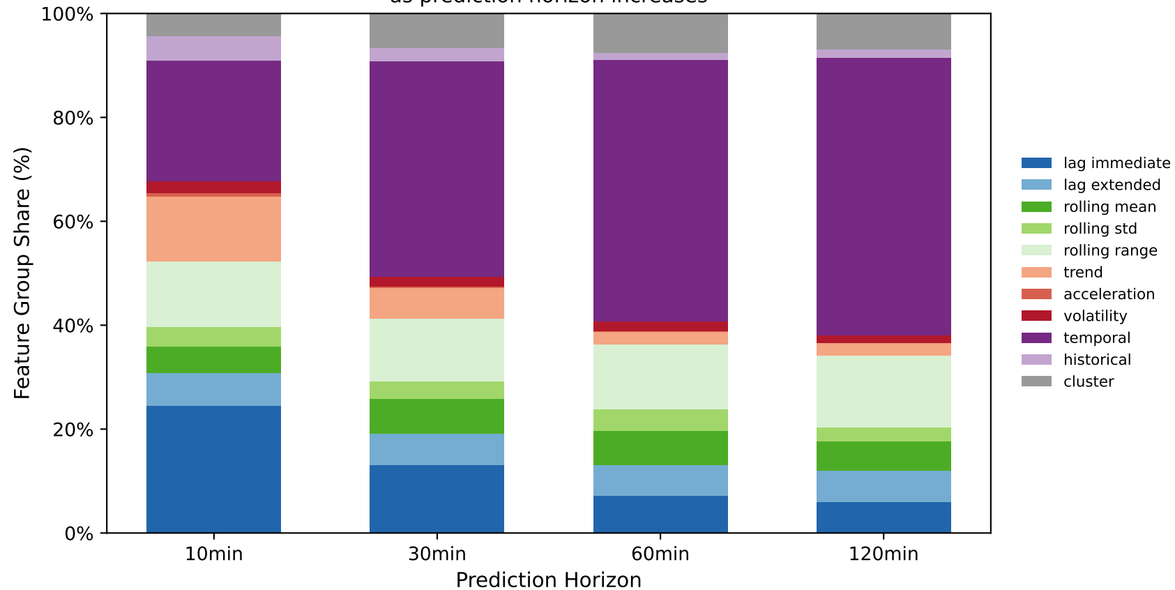
Feature importance shifts from lag-dominated to temporal-dominated as prediction horizon increases
