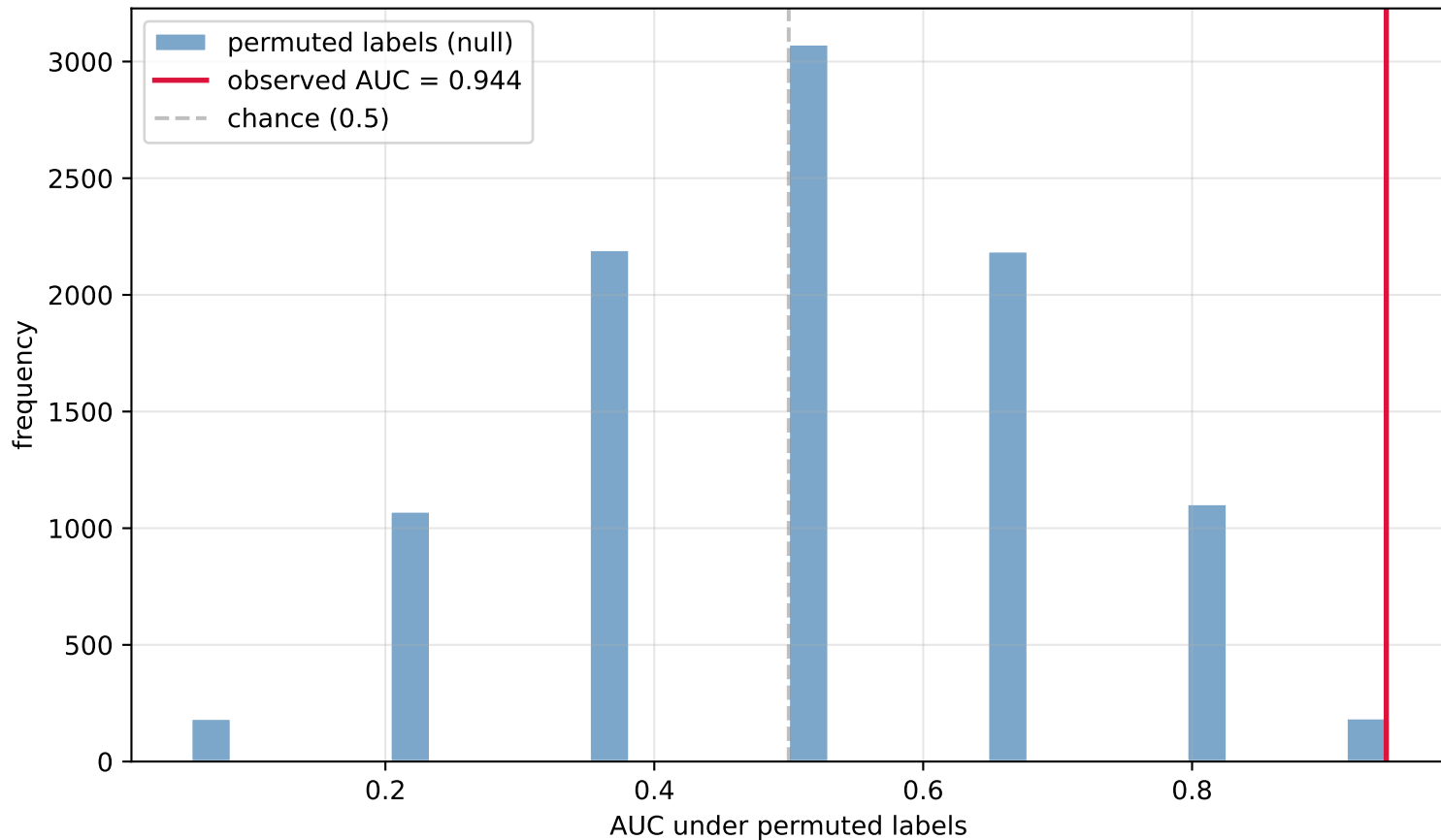
Permutation null distribution of AUC (n=12, 10000 perms, p=0.0186)
