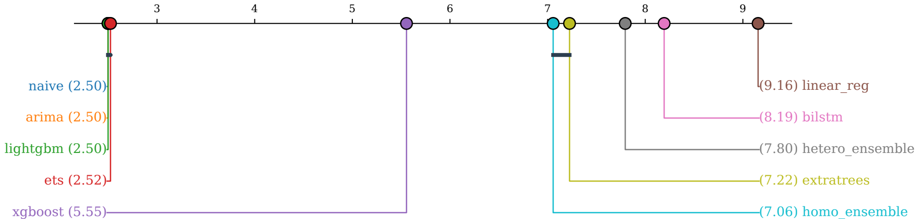
Critical difference diagram — 10min (n=4921 containers, Nemenyi \alpha=0.05 )
