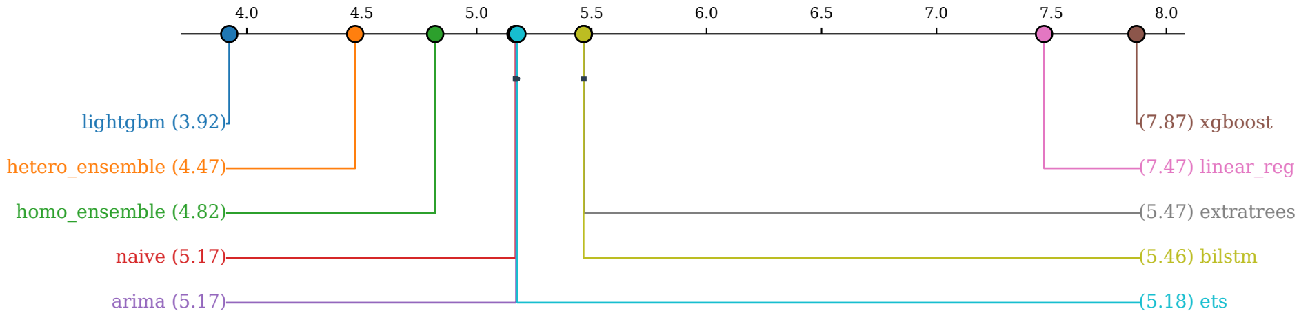
Critical difference diagram — 120min (n=4920 containers, Nemenyi \alpha=0.05 )
