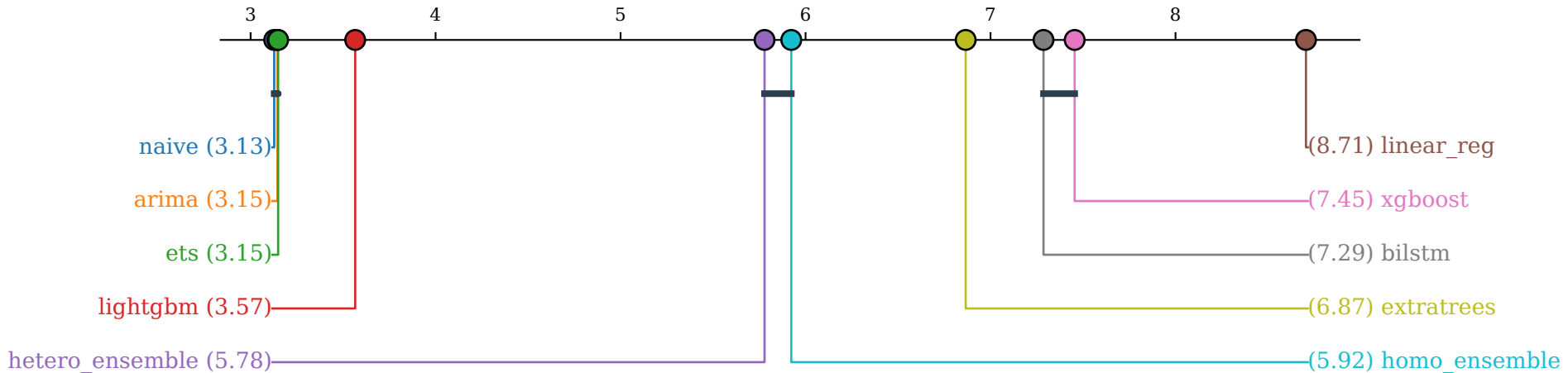
Critical difference diagram — 30min (n=4921 containers, Nemenyi \alpha=0.05 )
