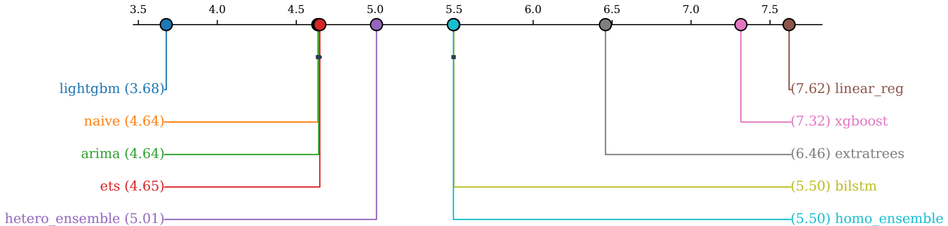
Critical difference diagram — 60min (n=4921 containers, Nemenyi \alpha=0.05 )
