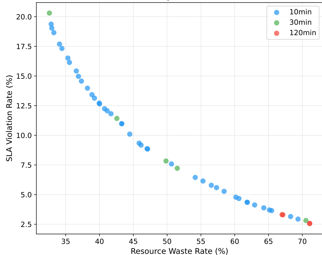
Pareto Front by Prediction Horizon
