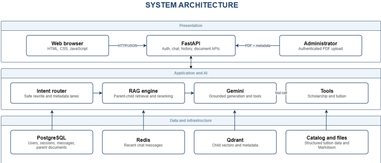
Figure 3.2. Application architecture
