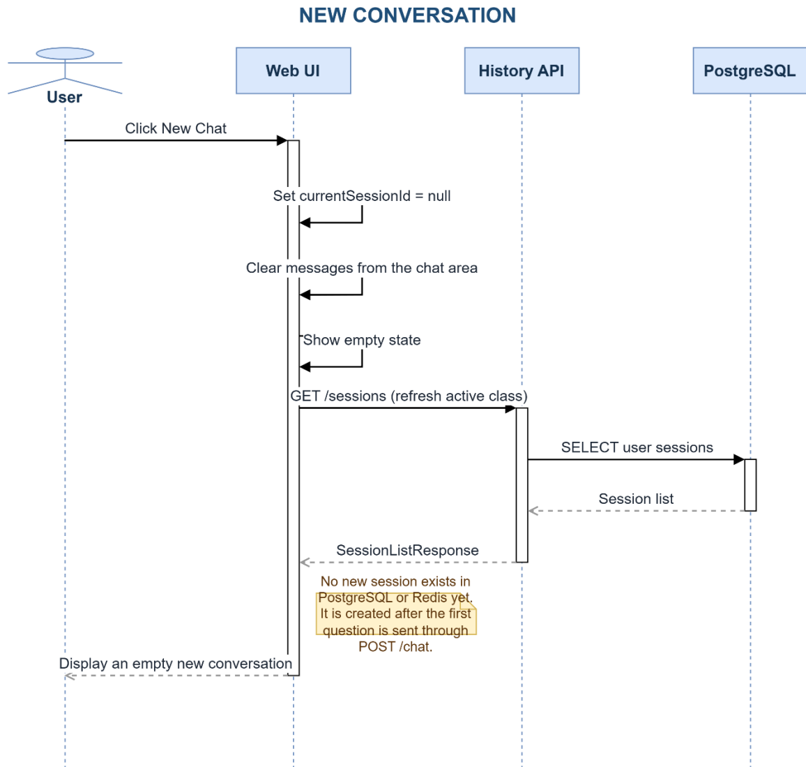
Figure 3.17. New Conversation sequence diagram
