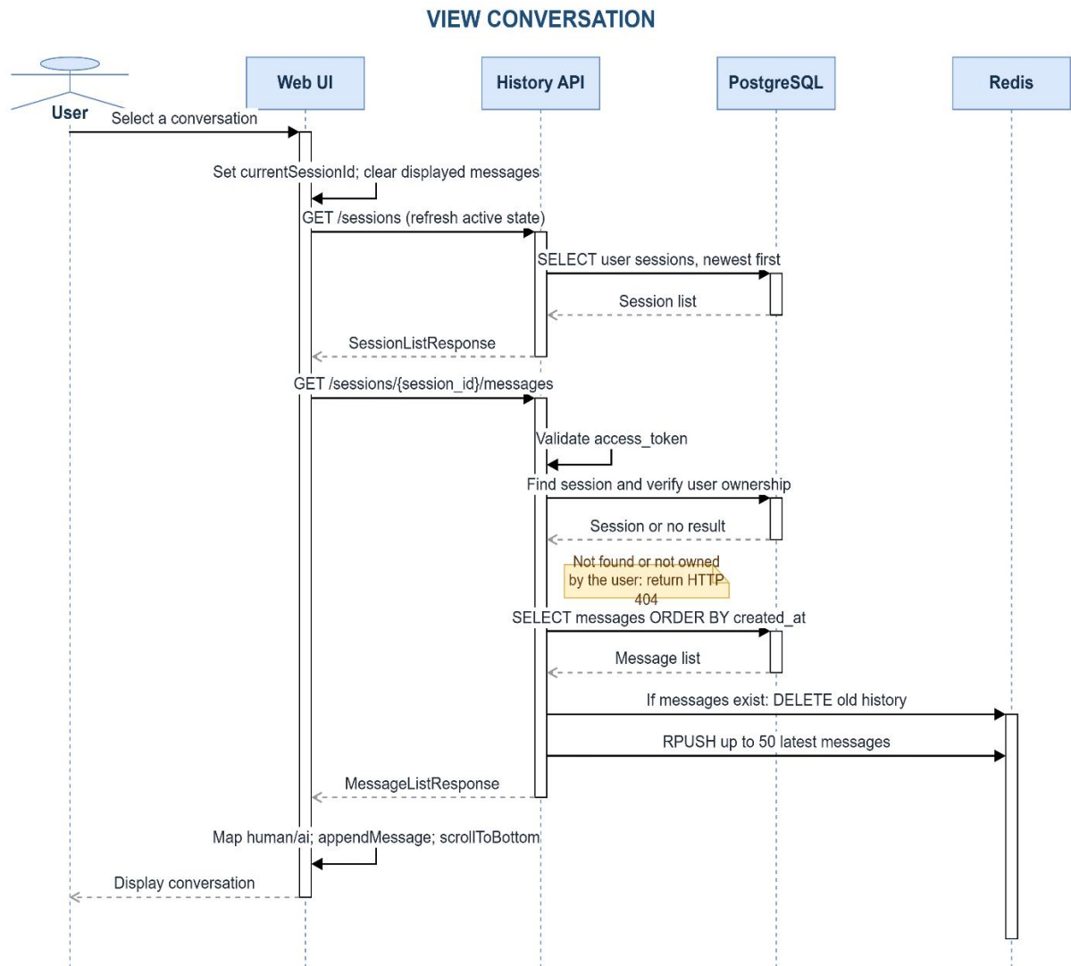
Figure 3.19. View Conversation sequence diagram
