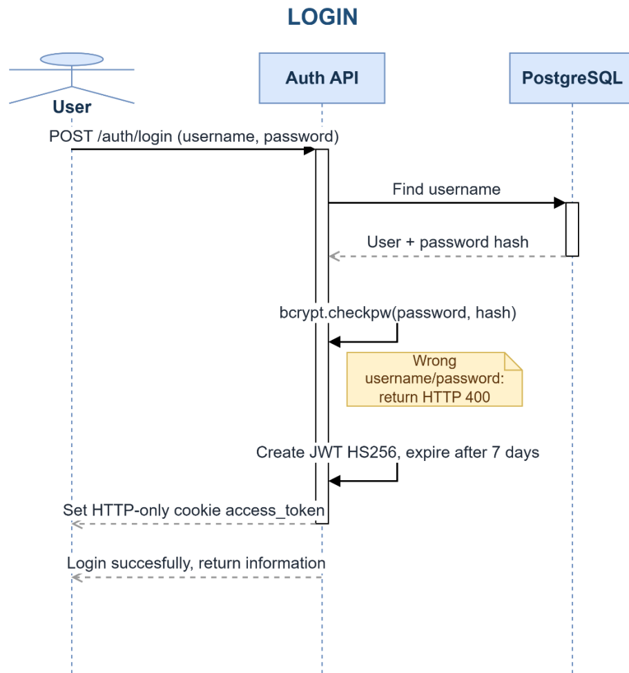
Figure 3.8. Login sequence diagram
