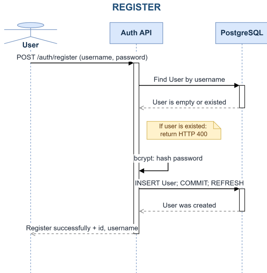
Figure 3.11. Registration sequence diagram
