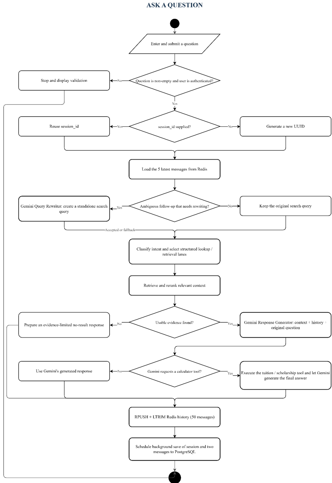
Figure 3.13. Ask a Question flowchart
