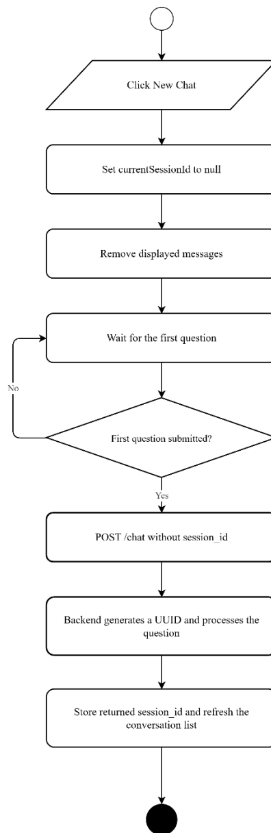
Figure 3.16. New Conversation flowchart
