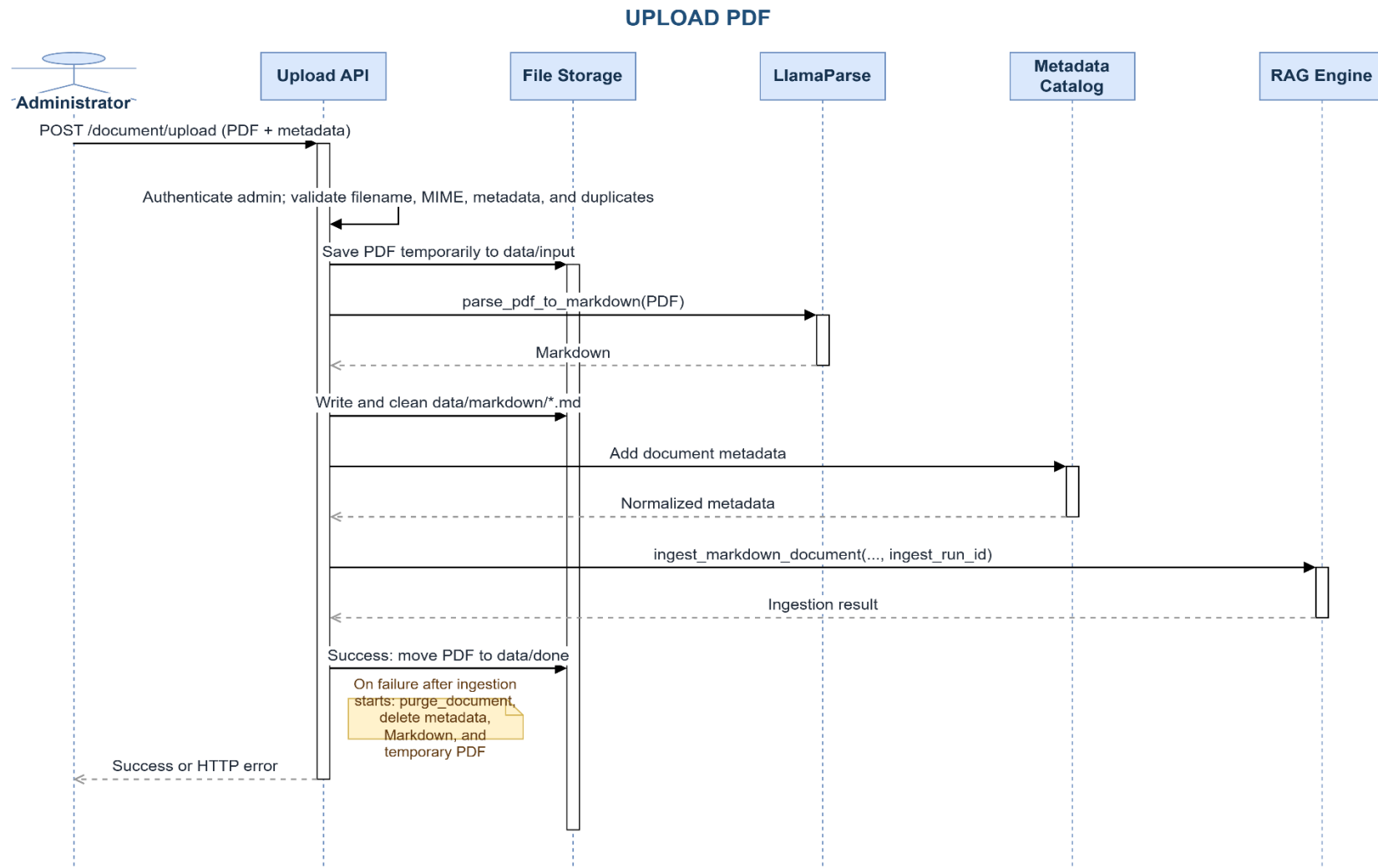
Figure 3.23. Upload PDF sequence diagram
