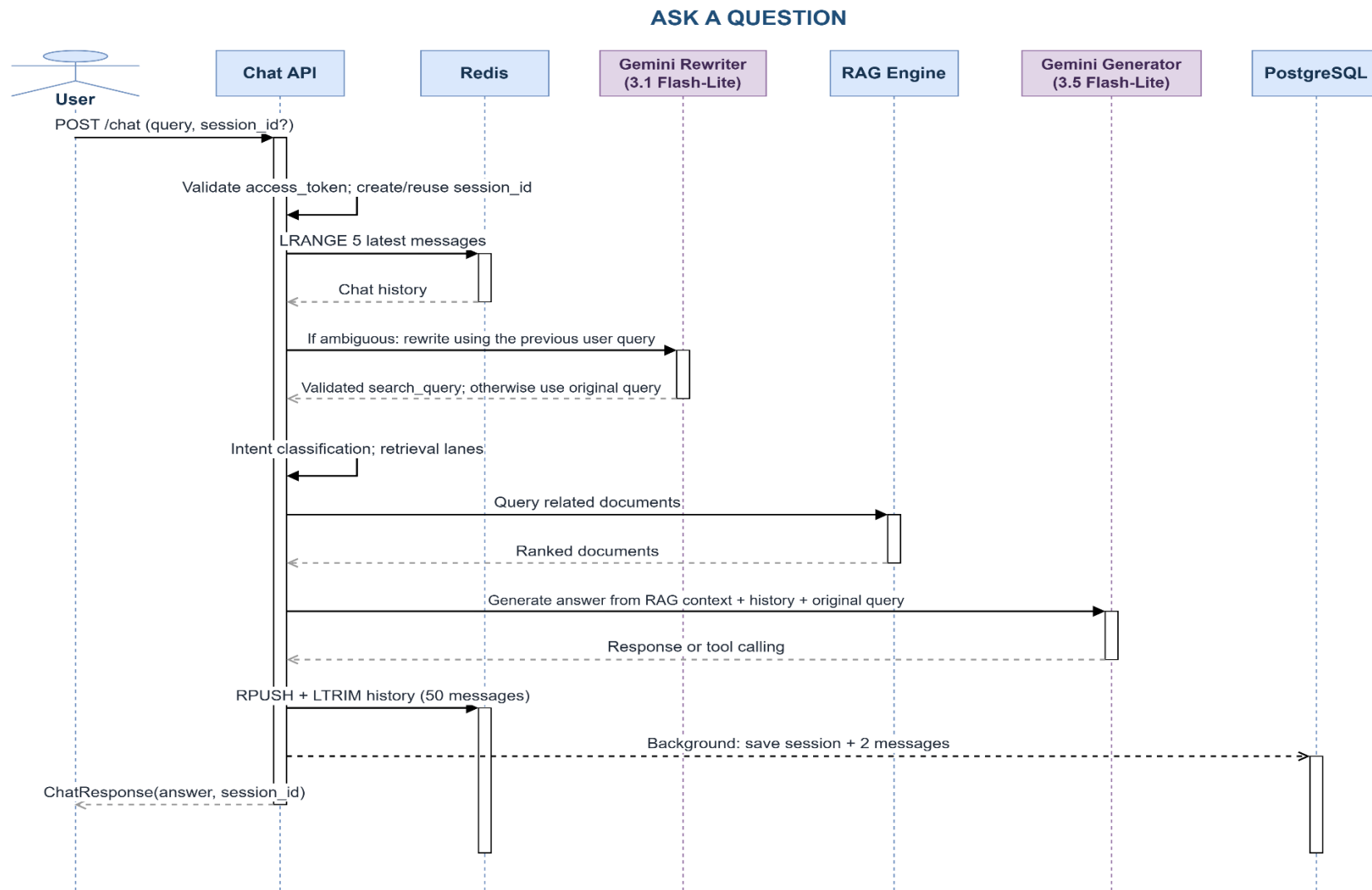
Figure 3.14. Ask a Question sequence diagram
