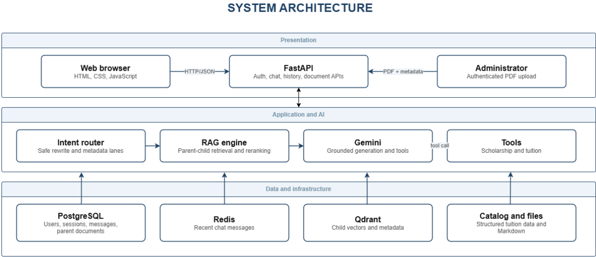
Figure 3.2. Application architecture
