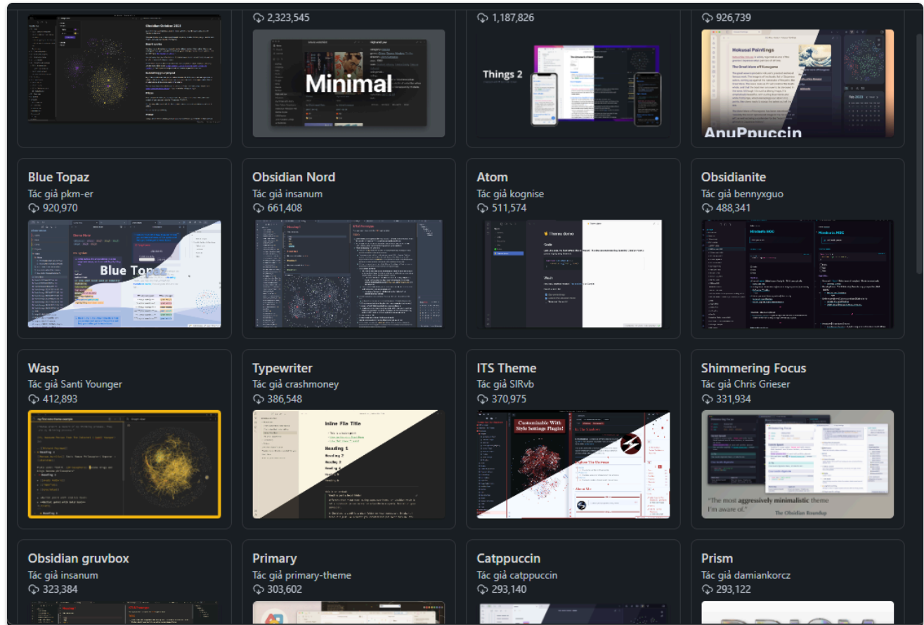
theme canvas
