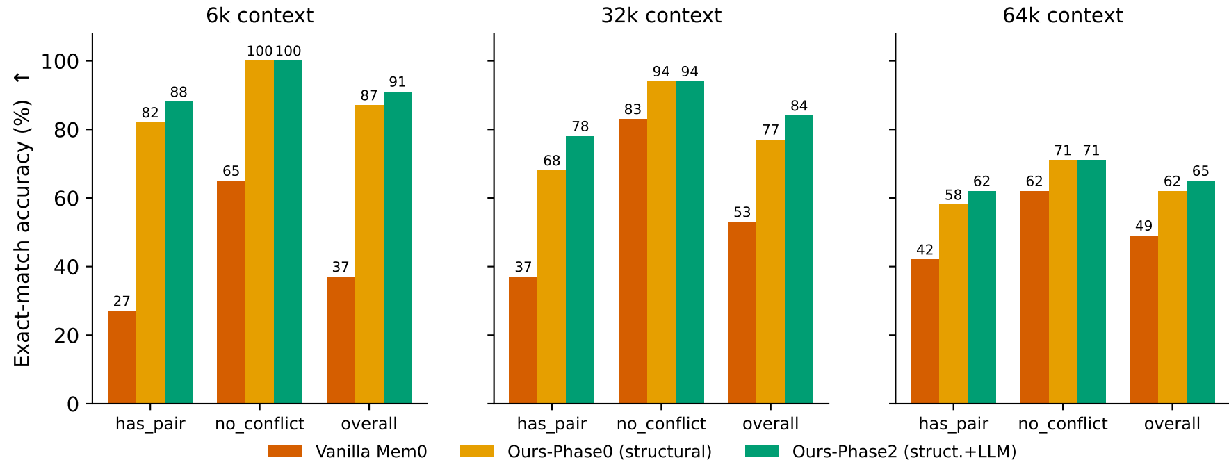
KU accuracy by conflict subset and history length
