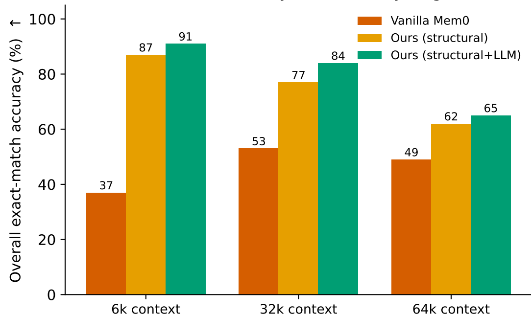
Overall KU accuracy across history lengths
