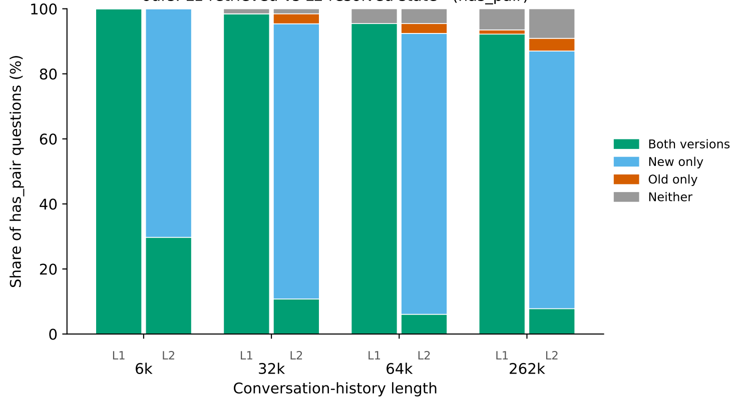
ours: L1 retrieved vs L2 resolved state (has_pair)
