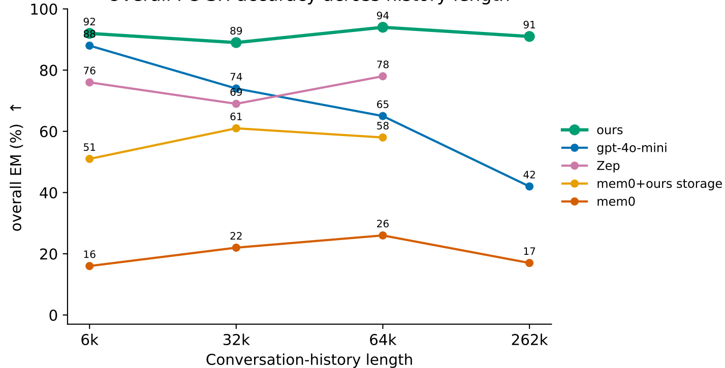
Overall FC-SH accuracy across history length
