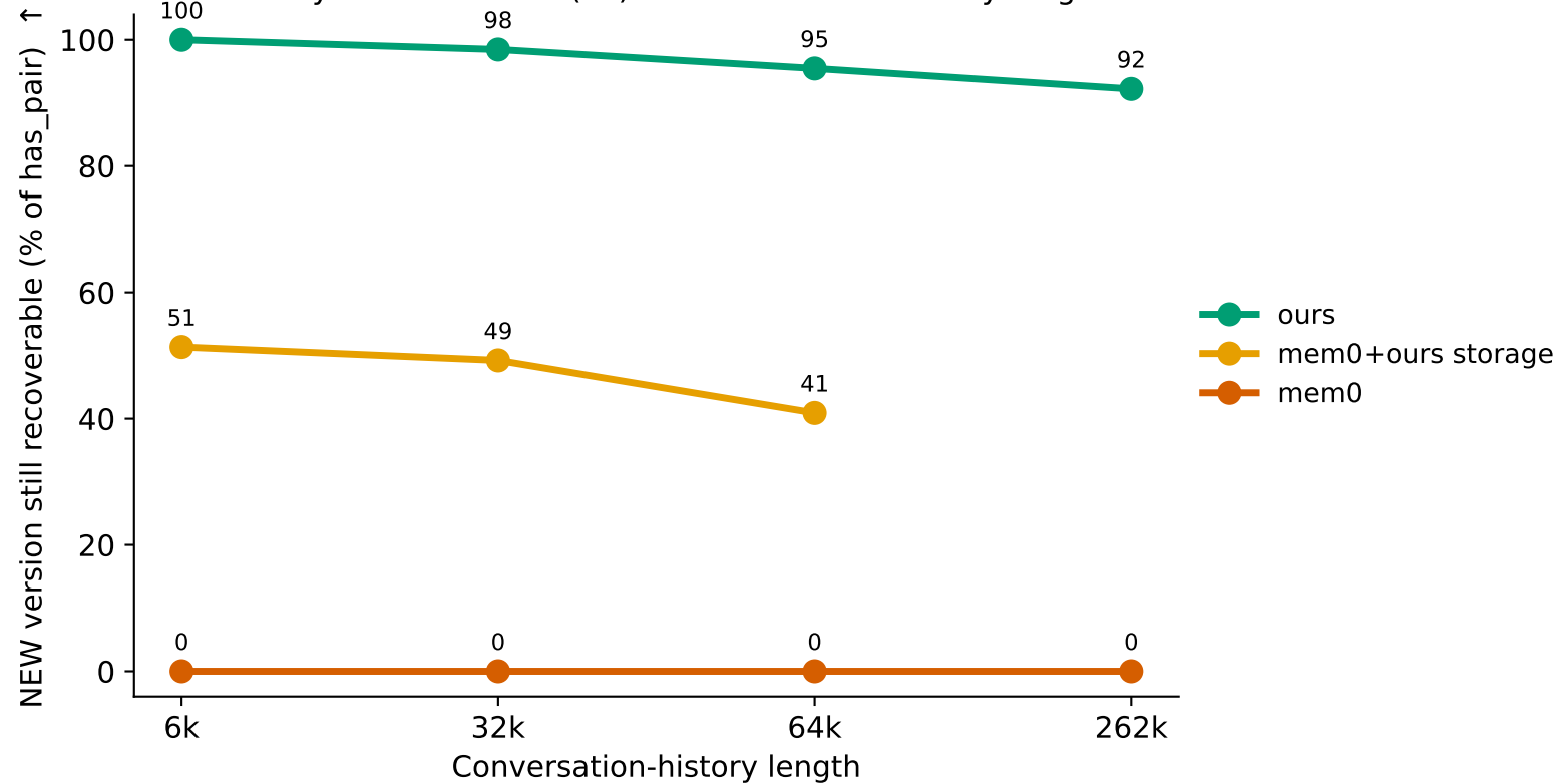
Memory-bank GT-recall (L0) vs conversation-history length
