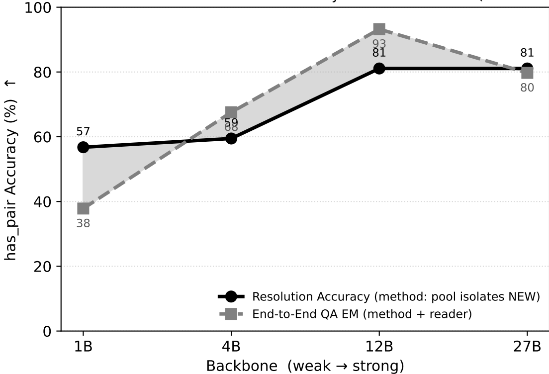
Method vs reader: Resolution Accuracy vs End-to-End EM (FC-SH 6k)
