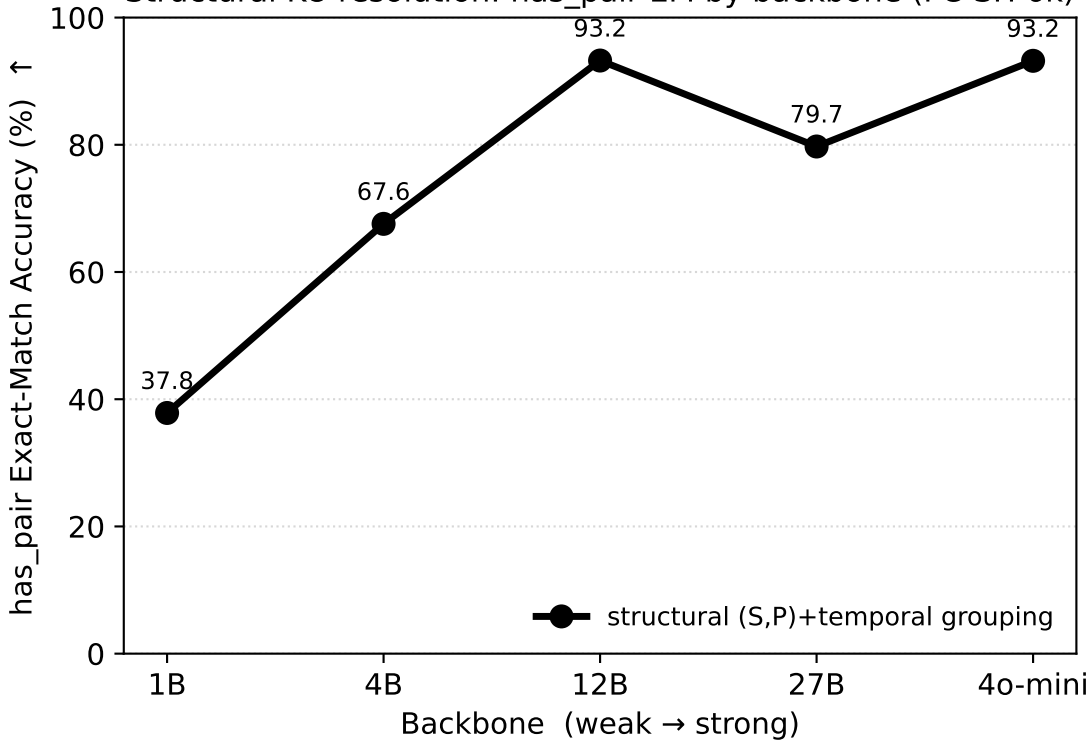
Structural KU resolution: has_pair EM by backbone (FC-SH 6k)
