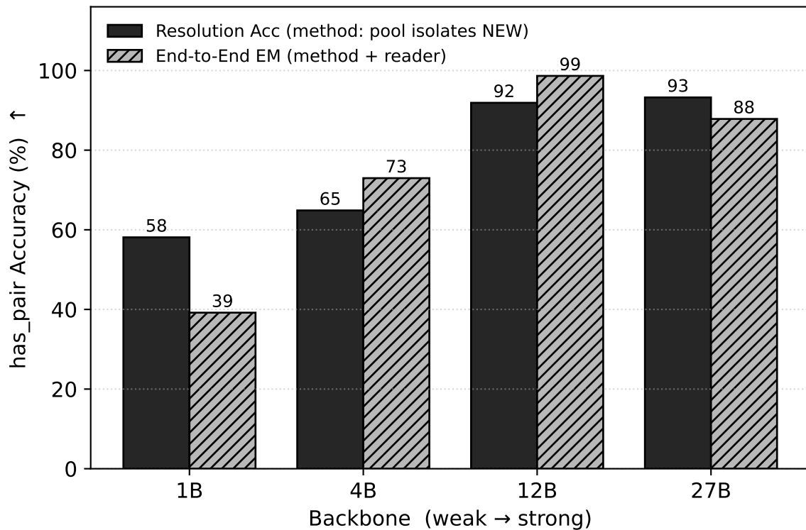
Method = ours_struct : structural (S,P) + deterministic temporal (no LLM grouping) FC-SH 6k has_pair, by backbone
