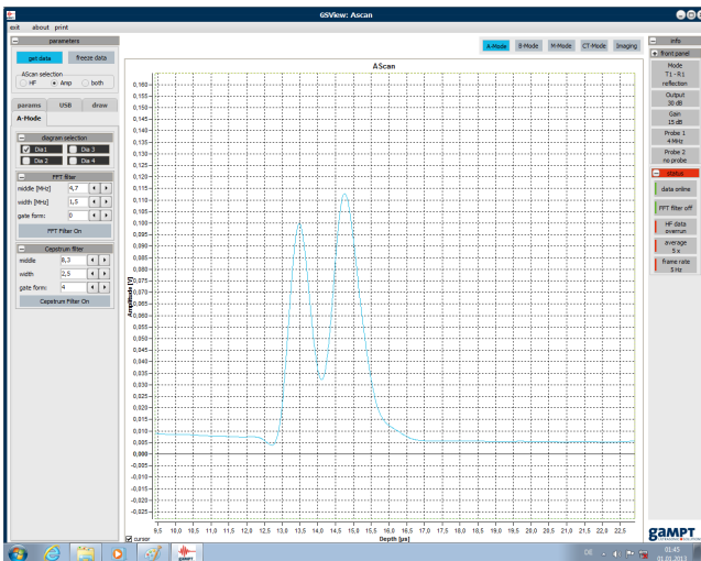
Figure 7: Shown is a screenshot of the A-scan hovering above hole 9a, 9b for the echoscope with 4MHz frequency
