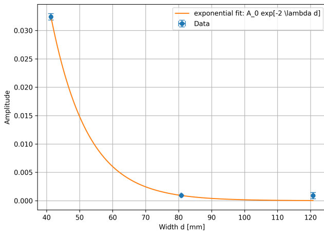
Figure 4: Exponential fit for the absorption with A_0 = 1.334 \pm 0.97 and \lambda = (0.4500 \pm 0.0080) \frac{1}{cm}
