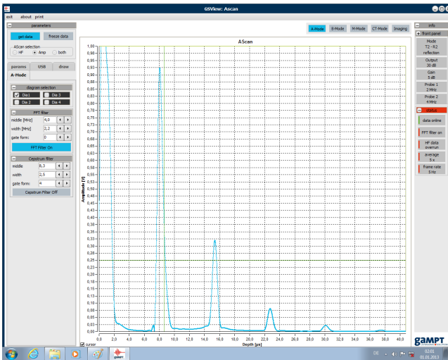
Figure 8: Shown is a screenshot of the A-scan with a FFT
