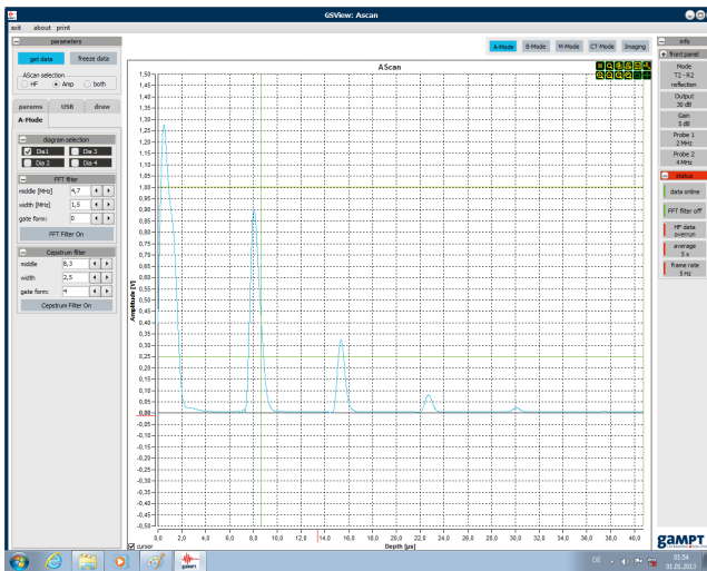
Figure 9: Shown is a screenshot of the A-scan with no FFT
