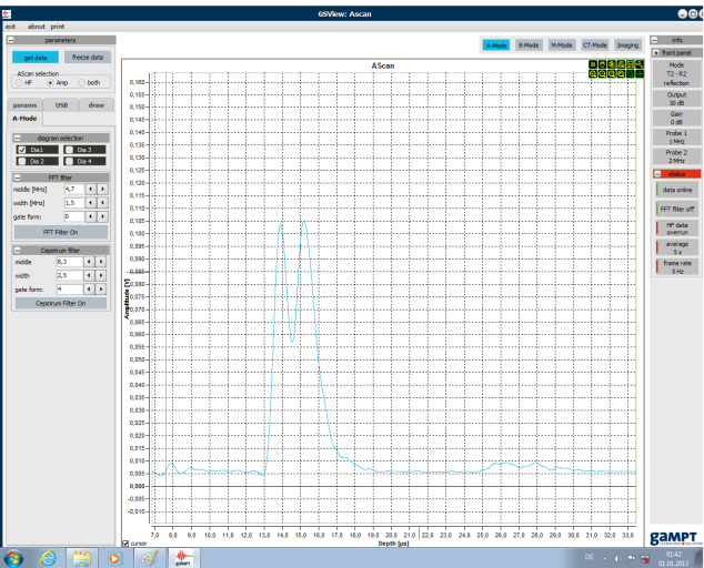
Figure 6: Shown is a screenshot of the A-scan hovering above hole 9a, 9b for the echoscope with 2MHz frequency
