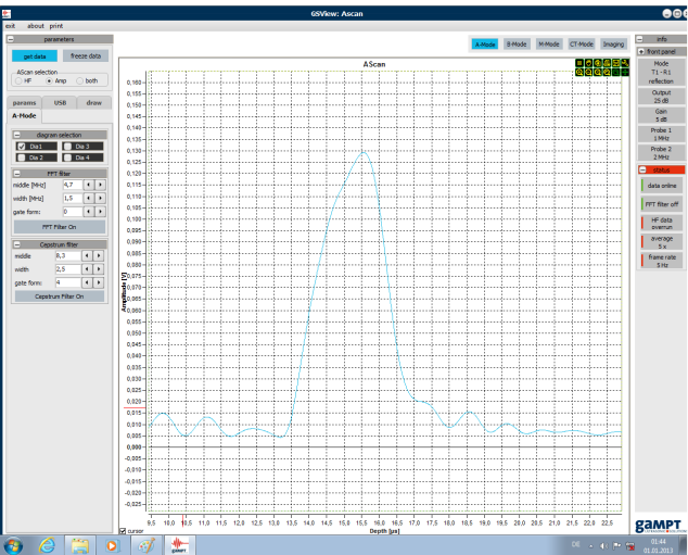
Figure 5: Shown is a screenshot of the A-scan hovering above hole 9a, 9b for the echoscope with 1MHz frequency
