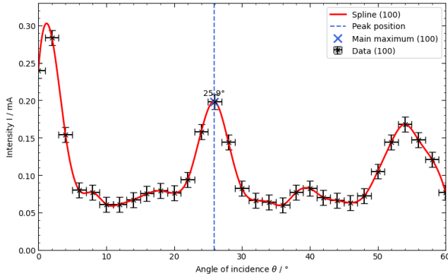
Figure 4: Measured Bragg diffraction from the (100) plane for angles \theta = [0, 60] . The first maximum was determined and marked.
