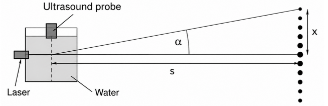
Figure 2: Setup used to measure the wavelength of ultrasound utilizing the Dabye-Sears effect
