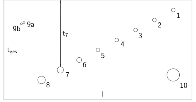
Figure 1: Schematics of the test block
