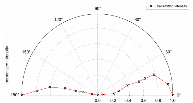
Figure 5: Polar plot of the normalized transmitted intensity as a function of the grid angle.
