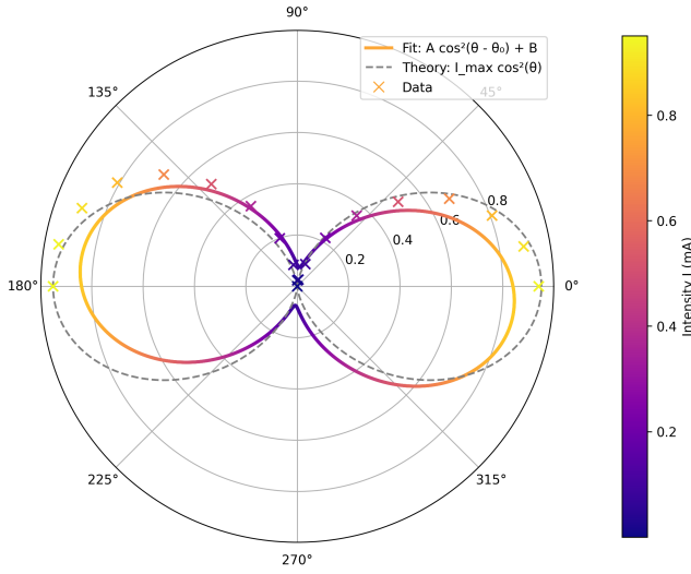
Figure 1: Measured intensity values and the fitted curve with fit I = A \cos^2(\theta - \theta_0) + B , A = 0.7720mA , \theta_0 = -5.95^\circ , B = 0.0761mA .
