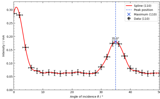
Figure 5: Measured Bragg diffraction from the (110) plane for angles \theta = [0, 50] . The first maximum was determined and marked.
