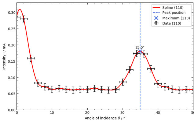
Figure 8: Measured Bragg diffraction from the (110) plane for angles \theta = [0, 50] . The first maximum was determined and marked.
