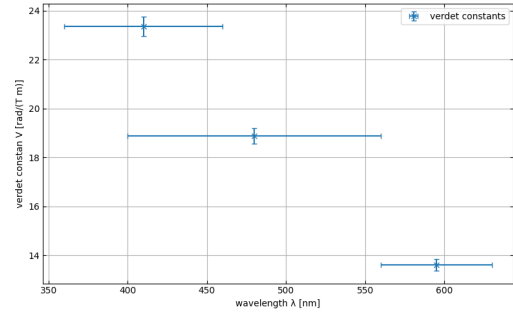
Figure 6: Dispersion of the Verdet constant as a function of the wavelength.
