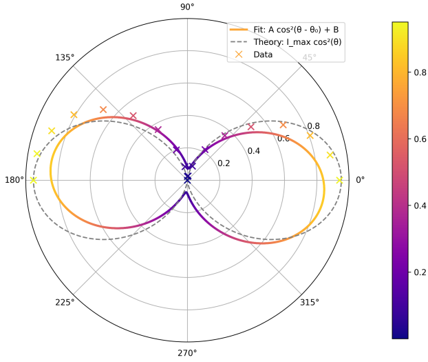
Figure 1: Measured intensity values and the fitted curve with fit I = A \cos^2(\theta - \theta_0) + B , A = 0.7720 \text{ mA} , \theta_0 = -5.95^\circ , B = 0.0761 \text{ mA} .
