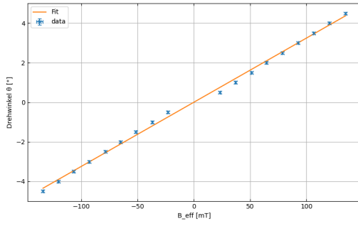
Figure 5: Rotation angle \Theta as a function of the effective magnetic field B_{\text{eff}} for the wavelength range 400–560 nm. The slope of the linear fit is used to calculate the Verdet constant.
