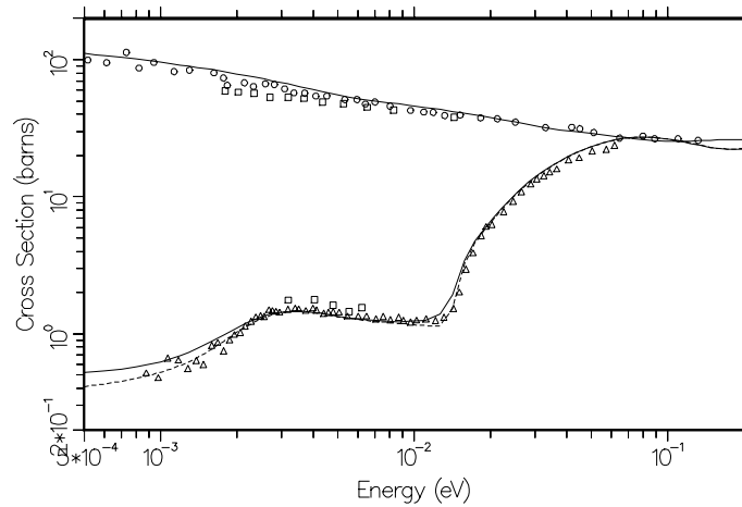
Figure 107: The cross sections for liquid ortho-hydrogen (upper curve) and liquid para-hydrogen (lower curve) at 20K are compared with experimental data[129] due to Squires (gas) at 20K (squares), Whittemore at 20K (circles), and Seiffert at 14K (triangles). The solid curves are at 20K and the dashed curve is at 14K. The sharp drop in the para cross section below 0.05 eV is due to spin coherence, and the second drop below 0.003 eV is due to intermolecular interference.
