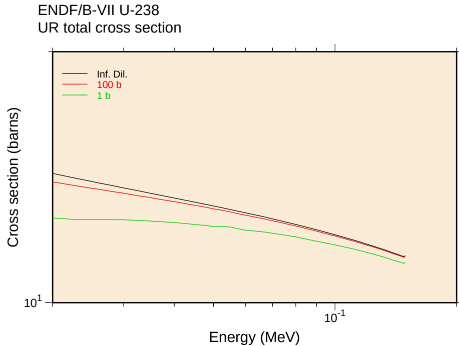
Figure 72: Bondarenko-style self-shielded cross sections for the total cross section of ^{238}\text{U} in the unresolved resonance region at three different dilutions.
