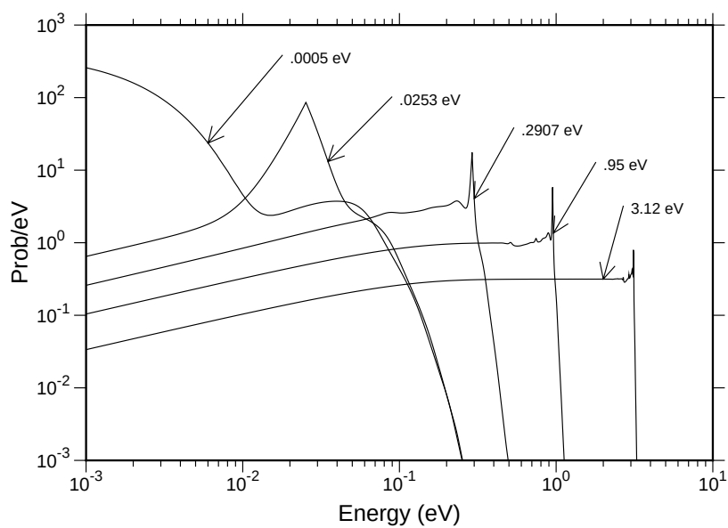
Figure 81: Incoherent inelastic spectra for several incident energies for H in H 2 O.
