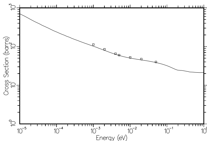
Figure 97: The computed cross section for liquid methane at 100K (solid) is compared to experimental data at 110K (squares) by Whittimore and by Rogalska as quoted by Agrawal and Yip.
