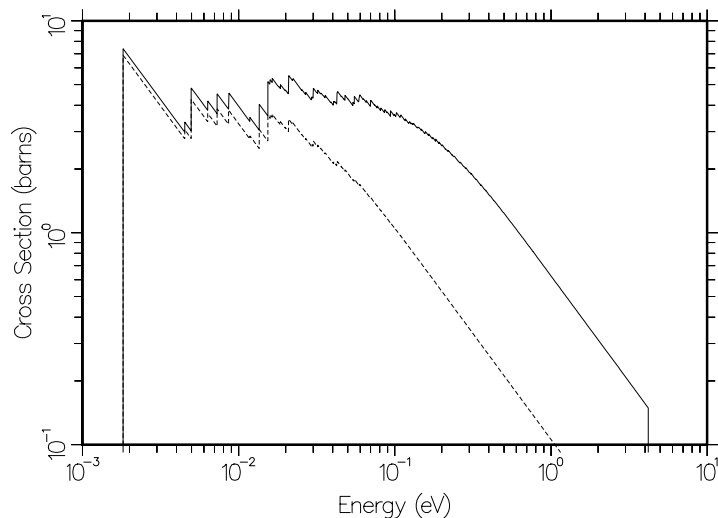
Figure 75: The coherent elastic cross section for graphite at temperatures of 293.6K (solid) and 2000K (dashed) showing the Bragg peaks. Note that the 293.6K cross section near the 4 eV breakpoint is still an appreciable part of the 4.74 barn free cross section.
