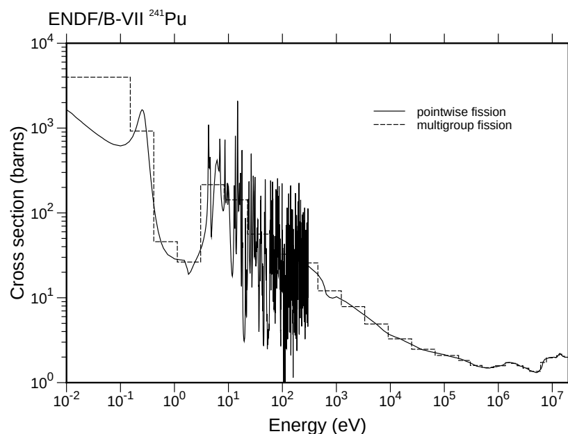
Figure 62: Comparison of the multigroup fission cross section of ENDF/B-VII.0 ^{241}\text{Pu} (dashed curve) with the corresponding pointwise cross section from the PENDF tape (solid curve).
