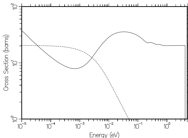
Figure 92: Inelastic (solid) and incoherent elastic (dashed) cross sections for solid methane. The small bumps starting at about 0.2 eV are due to the discrete levels at 0.162 eV, 0.190 eV, 0.361 eV, and 0.374 eV.
