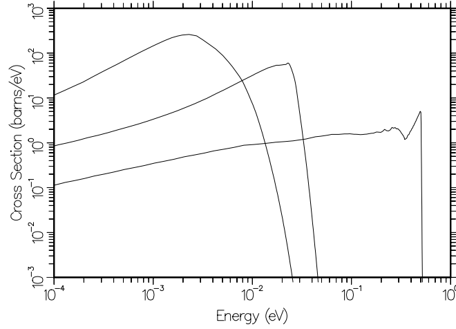
Figure 93: Neutron spectra \sigma(E \rightarrow E') for solid methane shown as functions of outgoing neutron energy E' for E = 0.0001 eV, 0.0253 eV, and 0.503 eV.
