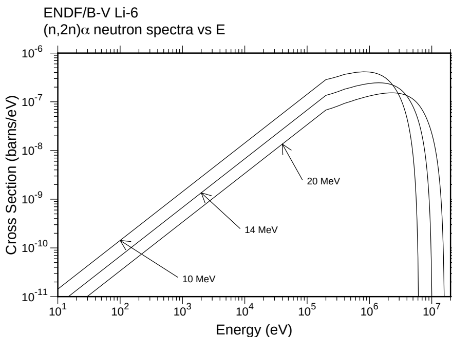
Figure 68: Two-D plot of selected secondary neutron spectra for the {}^6\text{Li} (n,2n) \alpha reaction.
