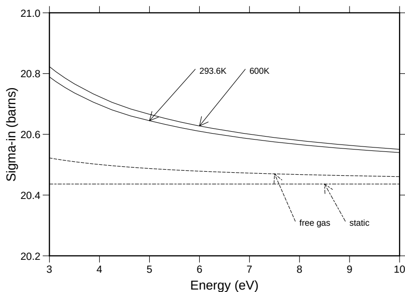
Figure 84: The incoherent inelastic cross section for H in \text{H}_2\text{O} for higher incident energies showing the static limit (scattering from atoms at rest) and the free-gas cross section.
