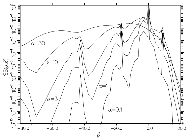
Figure 103: Script-S for ortho-hydrogen at 20K is shown as a function of \beta for several \alpha values.
