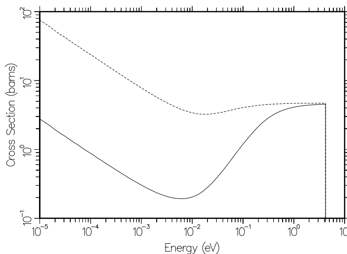
Figure 76: The incoherent inelastic cross section for graphite at temperatures of 293.6K (solid) and 2000K (dashed). A comparison of the two curves near the 4 eV breakpoint shows that the 293.6K cross section still has not reached the 4.74 barn free cross section. However, the sum of the elastic and inelastic components does equal the free value.
