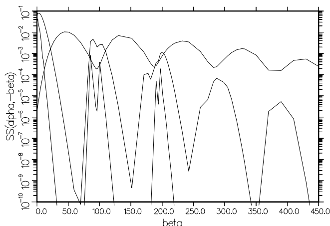
Figure 91: \mathcal{S}(\alpha, -\beta) for solid methane shown as a function of \beta for the \alpha values 0.986 (lowest), 16.94, and 151.45 (highest). The four discrete levels show up as sharp triangles in the lowest curve.
