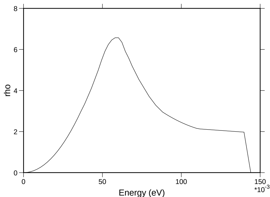
Figure 78: The frequency spectrum used for H in H 2 O for ENDF/B-VII.0.
