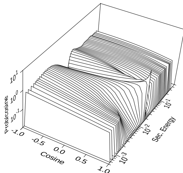
Figure 86: A perspective view of an angle-energy distribution for H in \text{H}_2\text{O} .
