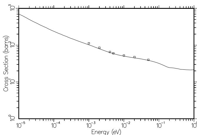
Figure 97: The computed cross section for liquid methane at 100K (solid) is compared to experimental data at 110K (squares) by Whitemore and by Rogalska as quoted by Agrawal and Yip.
