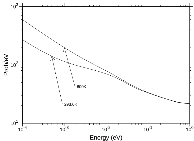
Figure 83: The incoherent inelastic cross section for H in \text{H}_2\text{O} at two temperatures.
