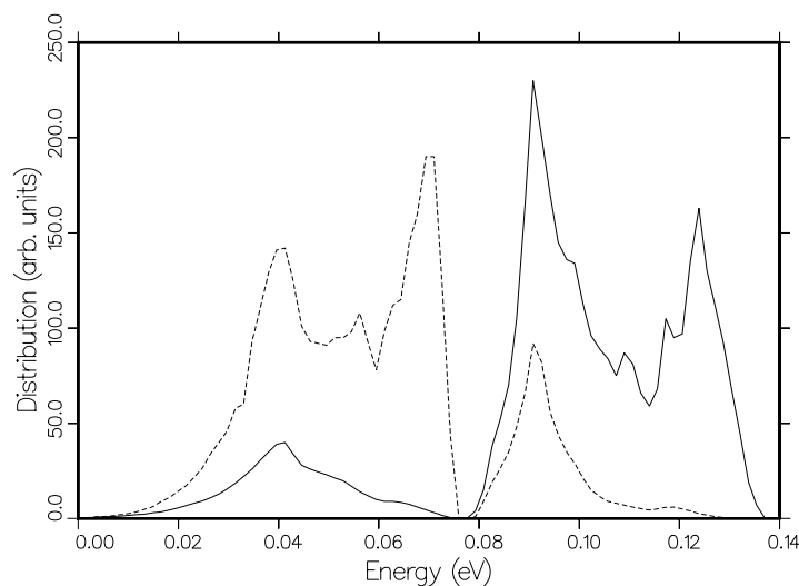
Figure 77: The frequency spectr \rho(\epsilon) used for Be in BeO (solid) and O in BeO (dashed).
