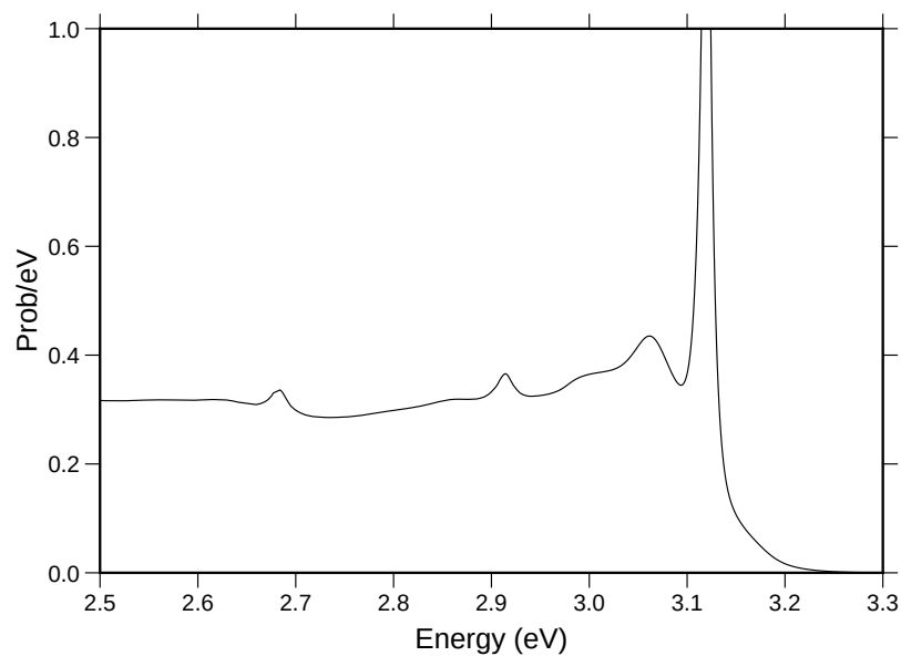
Figure 82: Detailed view of a neutron emission spectrum for inelastic scattering for H in \text{H}_2\text{O} .
