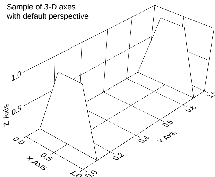
Figure 70: The 3-D coordinate system using the default work box and view point.
