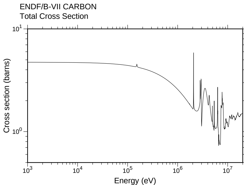
Figure 60: Simple 2-D plot of the total cross section of ENDF/B-VII carbon using log-log axes with user-selected ranges.
