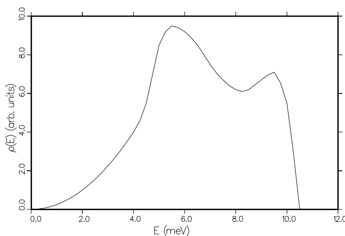
Figure 99: The Keinert-Sax frequency distribution for the effective translational modes of liquid hydrogen.
