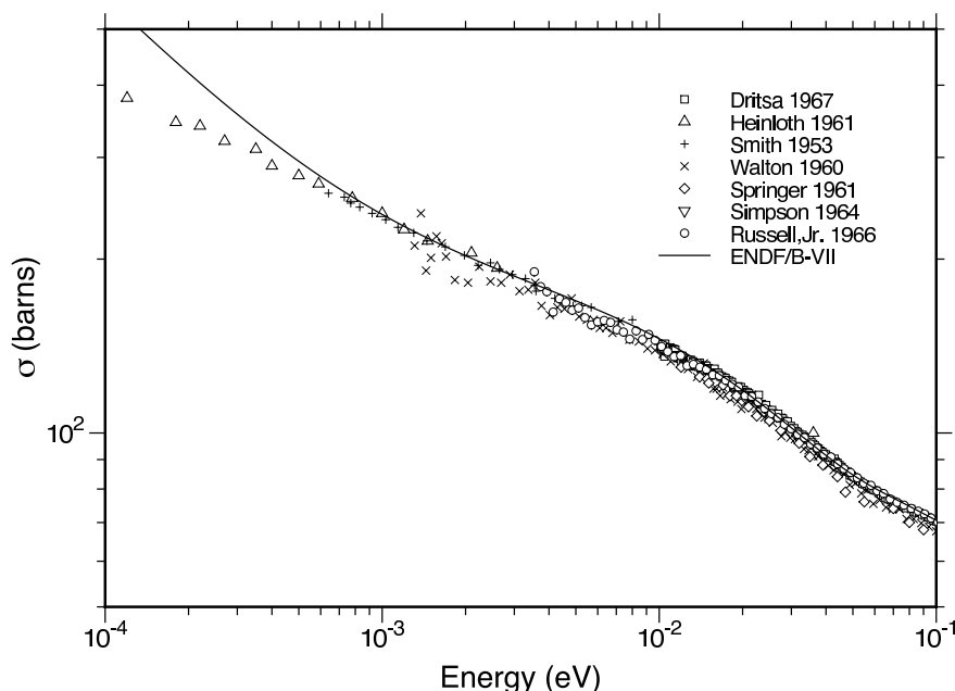
Figure 88: Comparison of the ENDF/B-VII.0 thermal cross section for water at lower incident energies with experimental results for the CSISRS compilation at the the National Nuclear Data Center of the Brookhaven National Laboratory. See the compilation for the references.
