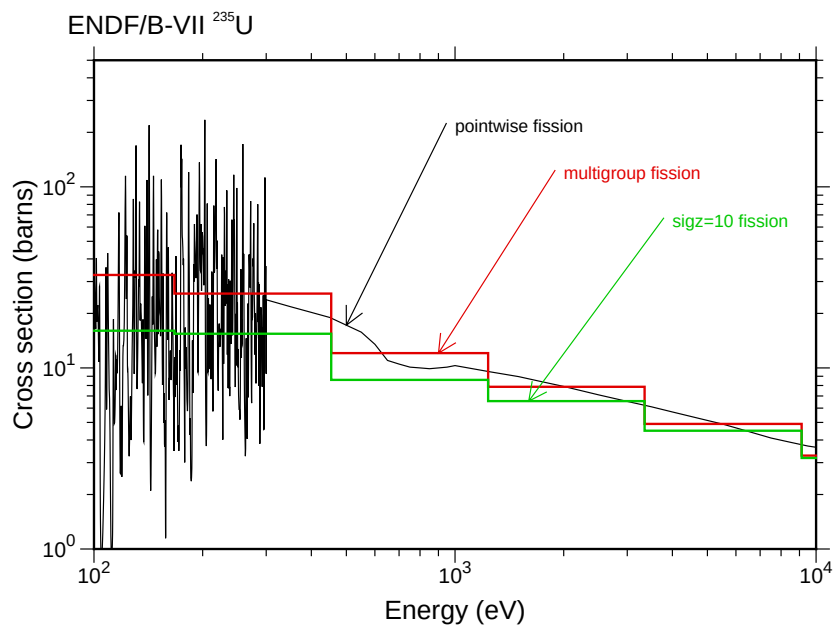
Figure 63: Multigroup fission cross sections of ENDF/B-VII.0 ^{235}\text{U} for infinite dilution and a 10-barn background compared with the corresponding pointwise cross section.
