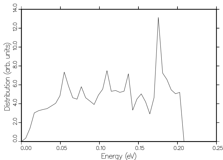
Figure 74: The phonon frequency spectrum \rho(\epsilon) used for graphite.
