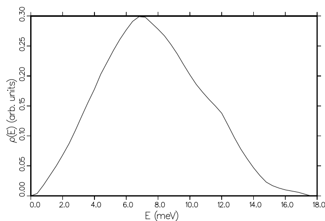
Figure 95: Effective frequency spectrum for methane including both translational and rotational modes, but not including diffusive modes.
