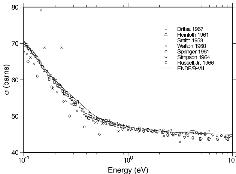
Figure 89: Comparison of the ENDF/B-VII.0 thermal cross section for water at higher incident energies with experimental results for the CSISRS compilation at the the National Nuclear Data Center of the Brookhaven National Laboratory. See the compilation for the references.
