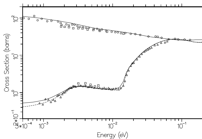
Figure 107: The cross sections for liquid ortho-hydrogen (upper curve) and liquid para-hydrogen (lower curve) at 20K are compared with experimental data[129] due to Squires (gas) at 20K (squares), Whittemore at 20K (circles), and Seiffert at 14K (triangles). The solid curves are at 20K and the dashed curve is at 14K. The sharp drop in the para cross section below 0.05 eV is due to spin coherence, and the second drop below 0.003 eV is due to intermolecular interference.
