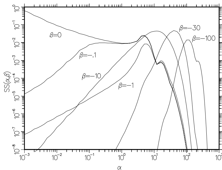
Figure 102: Script-S for para-hydrogen at 20K is shown as a function of \alpha for several \beta values corresponding to downscatter.
