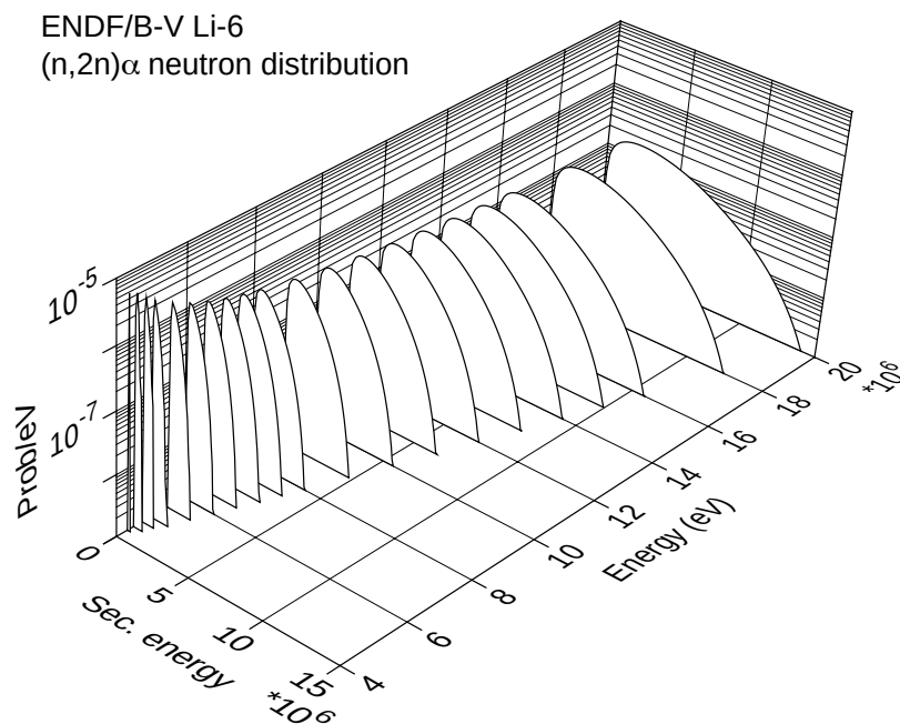
Figure 67: Perspective plot of {}^6\text{Li} (n,2n) \alpha neutron secondary-energy distributions.
