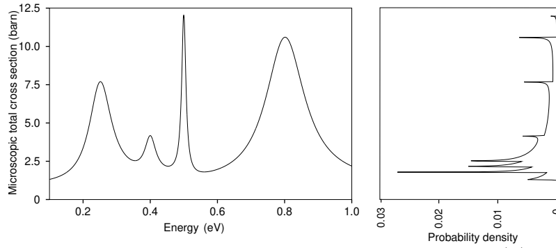
Figure 57: Representation of a probability density \Pi(\sigma) .
