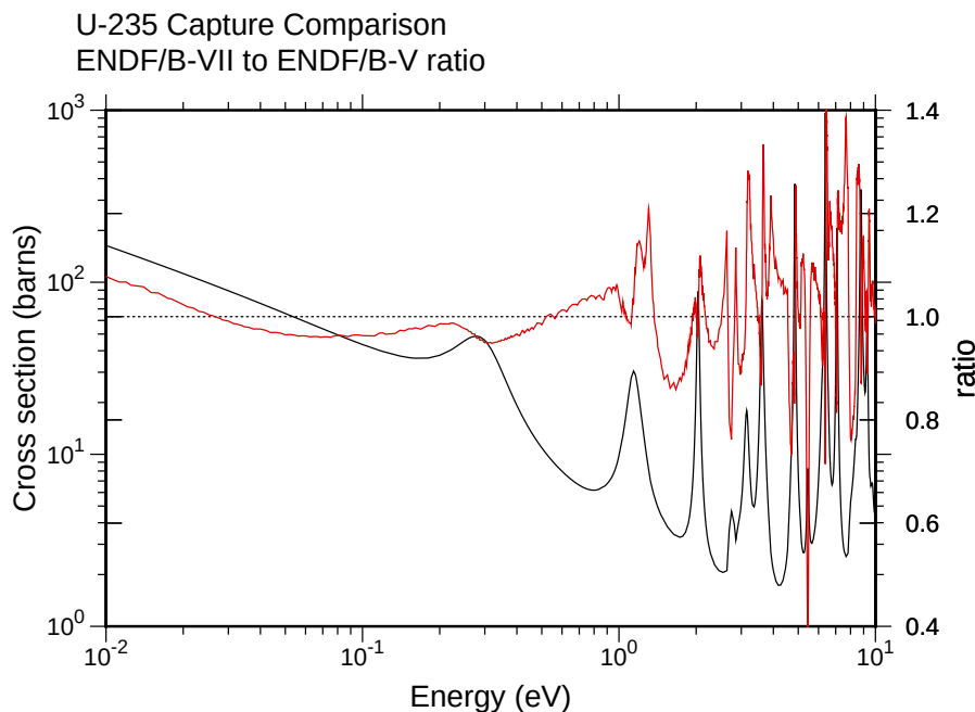
Figure 64: Using a right-hand axis to plot the ratio of the ENDF/B-VII.0 capture cross section for ^{235}\text{U} to the ENDF/B-V value. The black curve is the ENDF/B-V cross section, and the red curve is the ratio (right-hand axis).
