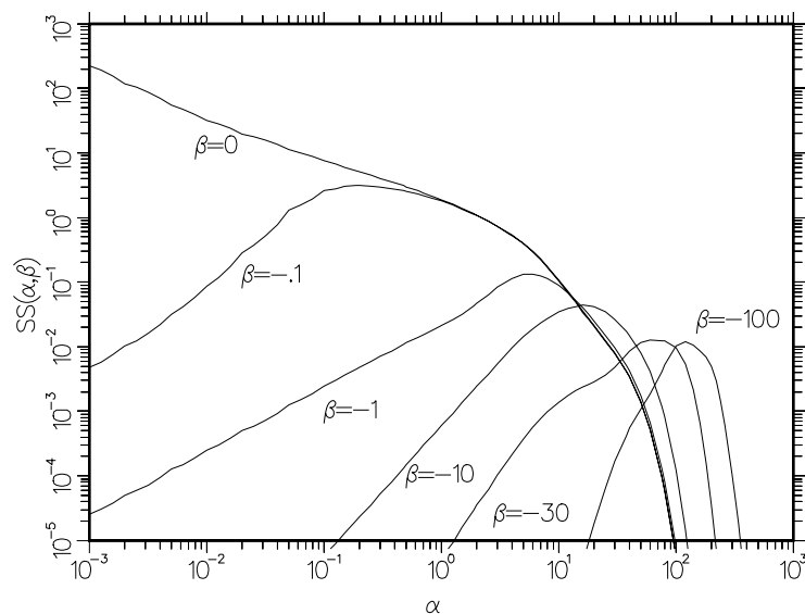
Figure 104: Script-S for ortho-hydrogen at 20K is shown as a function of \alpha for several \beta values corresponding to downscatter.
