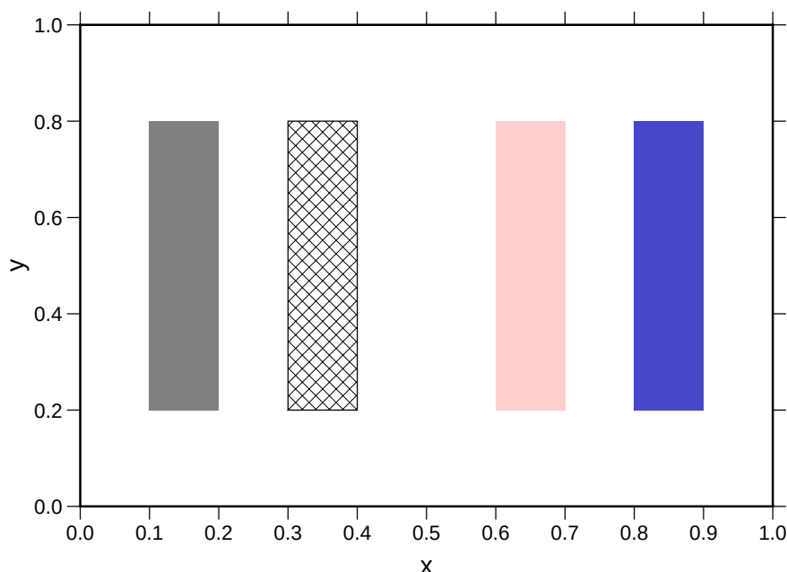
Figure 69: Examples of regions filled with gray, cross hatching and outlined, pink, and dark blue.
