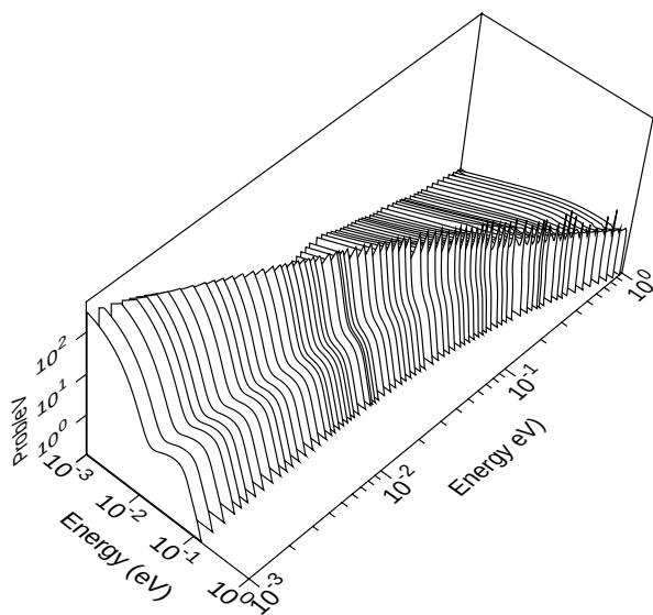
Figure 87: A perspective view of the isotropic part of the incoherent inelastic scattering from H in \text{H}_2\text{O} . The variations in the size of the quasi-elastic peak are artifacts of the plotting program.
