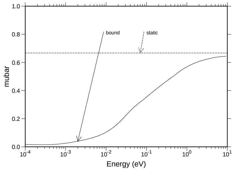
Figure 85: The average scattering cosine for H in H 2 O compared to the static value for scattering from atoms at rest. The effect of the binding of H in H 2 O is to make the scattering more isotropic at thermal energies.
