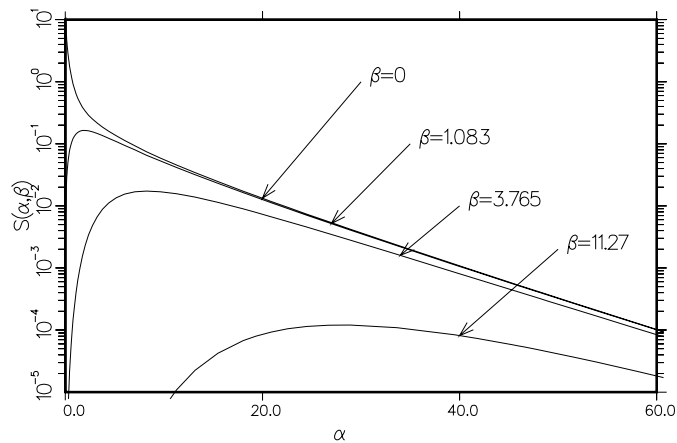
Figure 96: S(\alpha, \beta) curves for liquid methane. Note the diffusive behavior at low \alpha and \beta .
