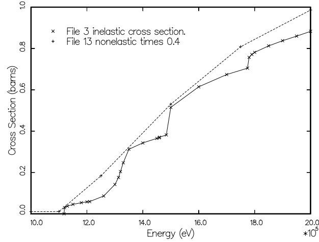
Figure 13: Plot showing the mismatch between the energy grids used for File 3 and File 13 in the region of the thresholds for discrete-inelastic scattering levels for the case shown in Fig. 12. The cross and ex symbols show the actual grid energies in the evaluation.
