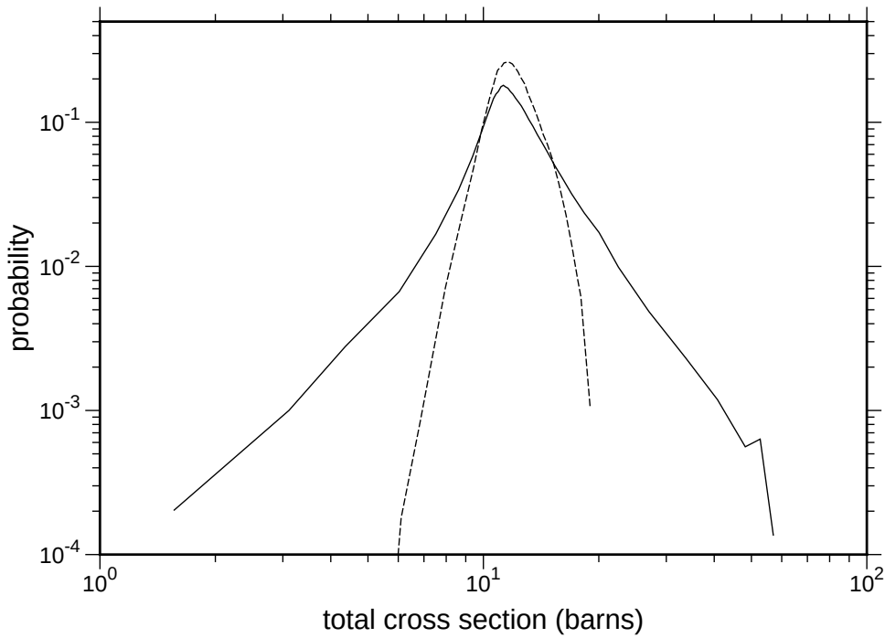
Figure 71: The probability distribution for the total cross section at 20 keV (solid) and 140 keV (dashed) in the unresolved resonance range of ^{238}\text{U} .
