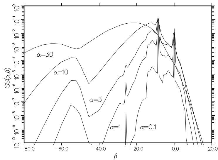
Figure 101: Script-S for para-hydrogen at 20K is shown as a function of \beta for several \alpha values.
