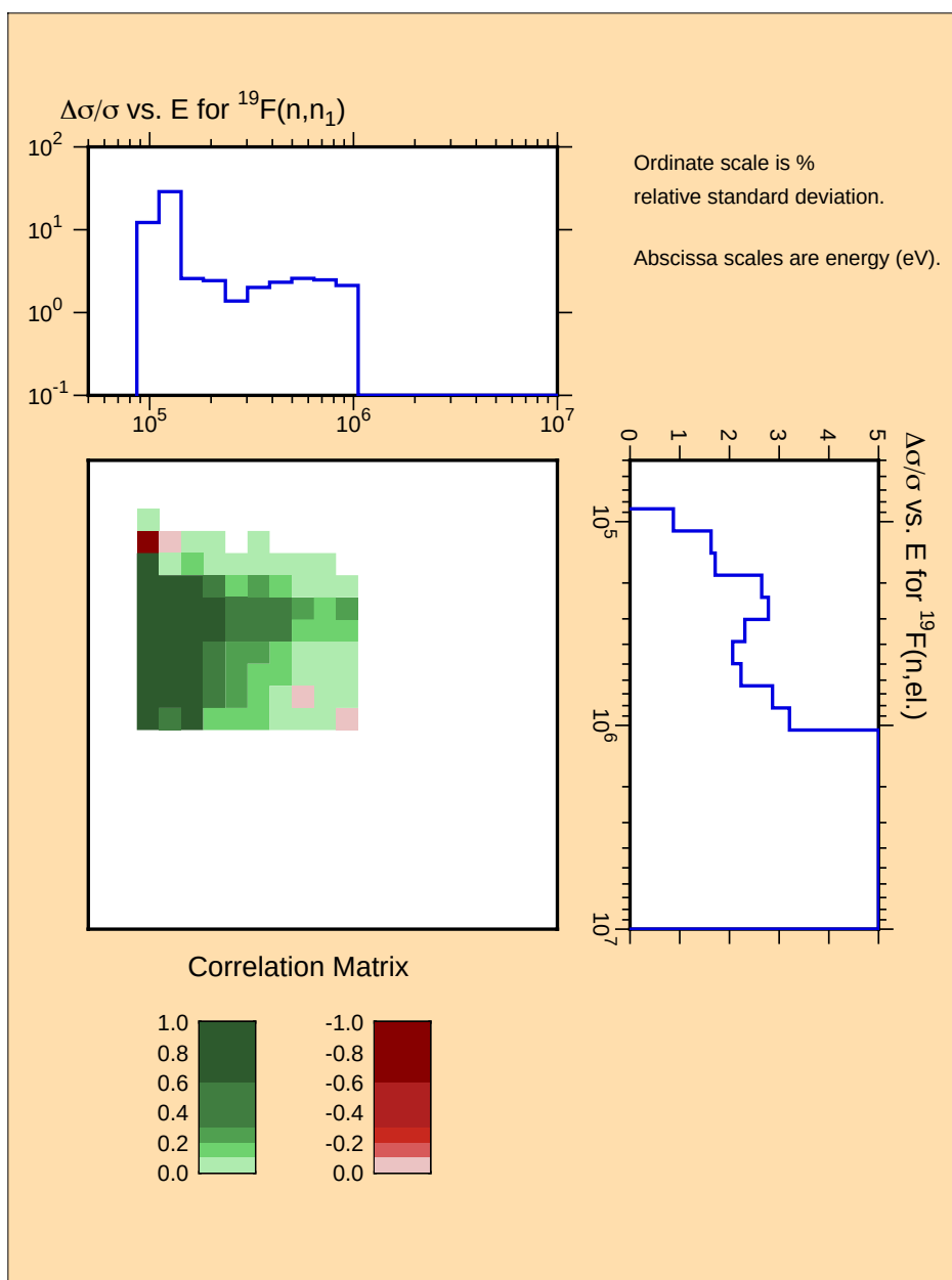
Figure 39: Covariance plot for the elastic and (n,n 1 ) reactions from a sample ORNL evaluation for ^{19}\text{F} , demonstrating the channel-channel covariances possible when using the Reich-Moore-Limited resonance representation.
