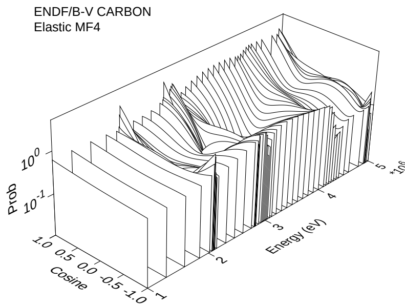
Figure 66: Perspective view of carbon elastic scattering angular distribution.
