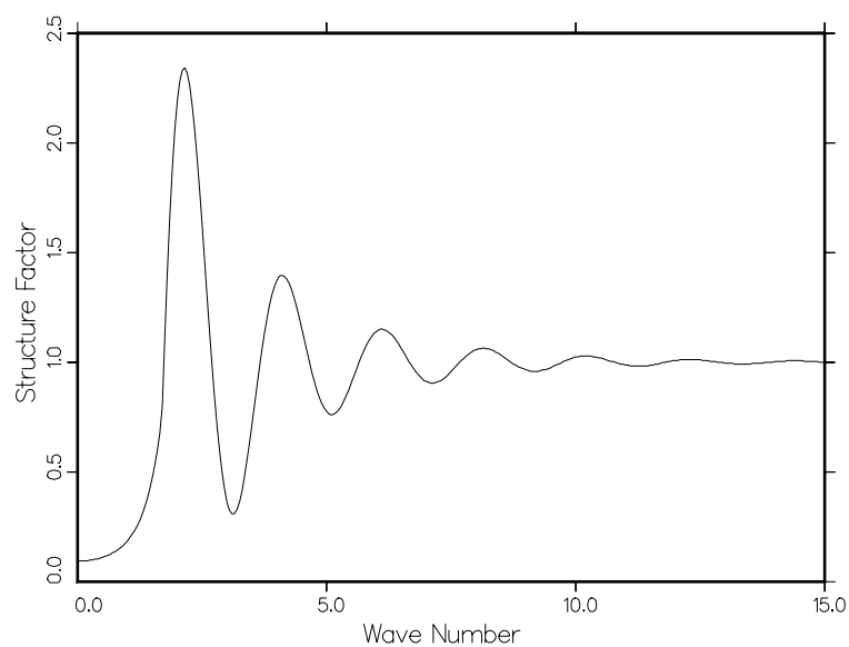
Figure 100: The static structure factor S(\kappa) for liquid hydrogen.
