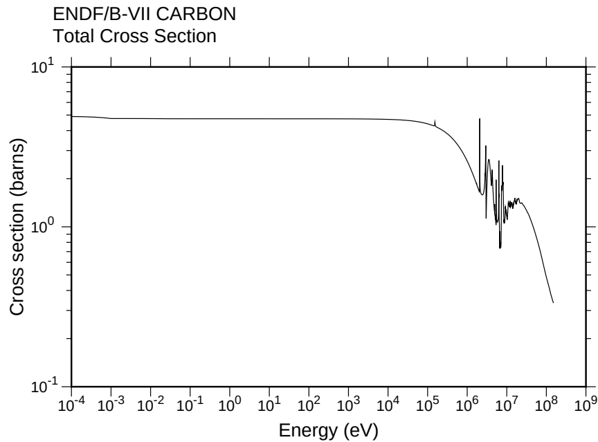
Figure 59: Simple 2-D plot of the total cross section of ENDF/B-VII carbon using automatic log-log axes.
