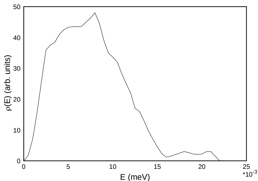
Figure 90: The Harker-Brugger frequency spectrum used for solid methane. Note the quadratic shape at low energies.
