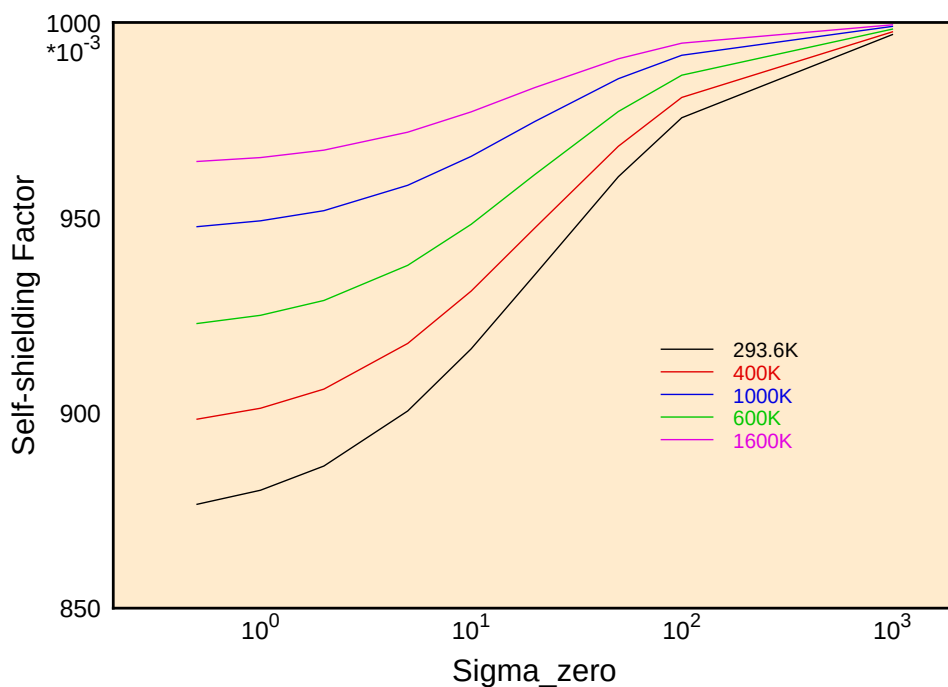
Figure 73: Self-shielding factors for the total cross section of ^{238}\text{U} at 20 keV showing the variation with temperature and background cross section (dilution).
