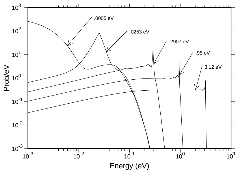
Figure 81: Incoherent inelastic spectra for several incident energies for H in H 2 O.
