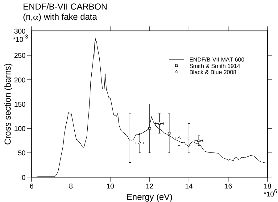
Figure 65: Carbon (n,α) cross section compared with two sets of simulated experimental data represented with two types of error bars.
