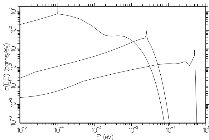
Figure 98: Neutron spectra \sigma(E \rightarrow E') are shown for E = 0.0001 eV, 0.0253 eV, and 0.503 eV. Note the sharp quasi-elastic peak that results from the diffusive term in the theory used here.
