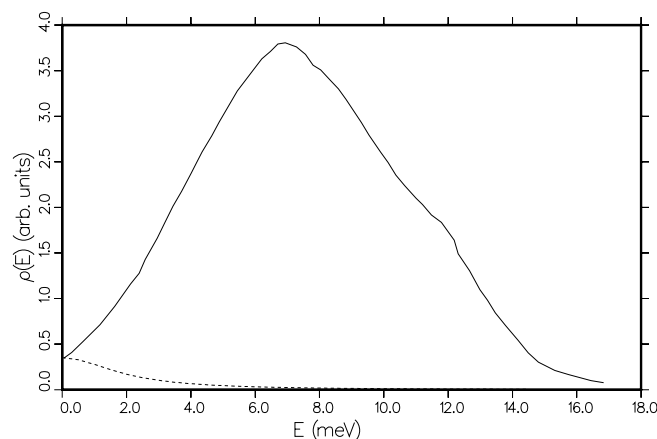
Figure 94: Frequency spectrum for liquid methane (solid) as given by Agrawal and Yip, including an analytic translational part (dashed) and a rotational part based on Gordon’s analysis of the optical measurements of Ewing.
