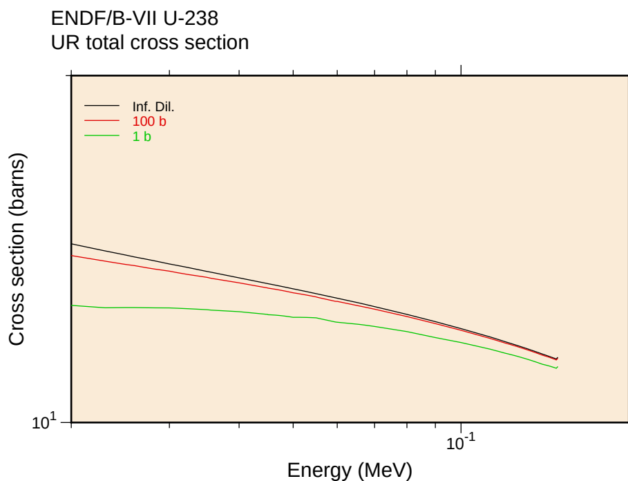
Figure 72: Bondarenko-style self-shielded cross sections for the total cross section of ^{238}\text{U} in the unresolved resonance region at three different dilutions.
