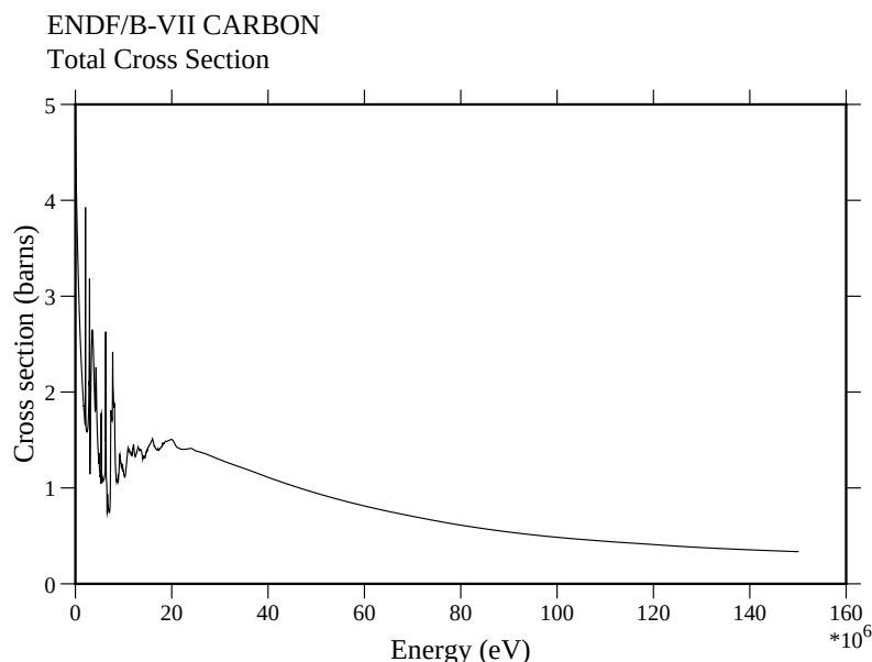
Figure 61: Simple 2-D plot of the total cross section of ENDF/B-VII.0 carbon using linear axes to emphasize the high-energy region and a more elaborate font.
