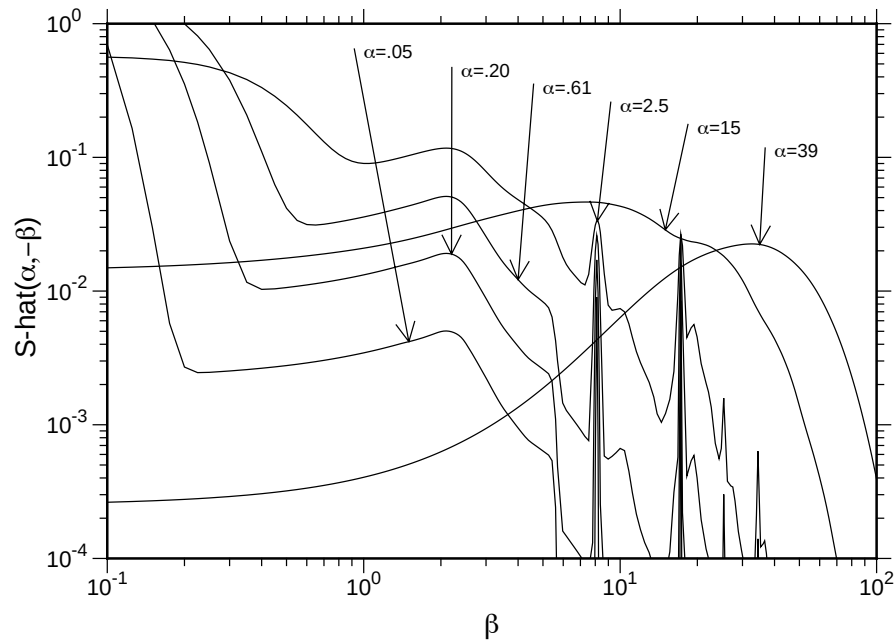
Figure 79: \mathcal{S}(\alpha, -\beta) for H in H 2 O at room temperature plotted versus \beta for various values of \alpha .
