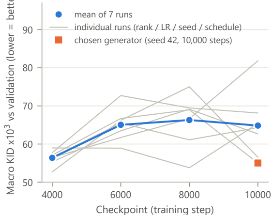
b Generator quality by checkpoint: large run-to-run swings
