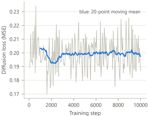
a Baseline LoRA training loss: flat
