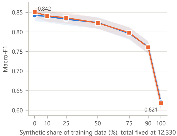
b Replacing real with synthetic: macro-F1
