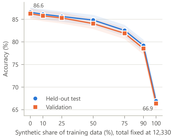
a Replacing real with synthetic: accuracy
